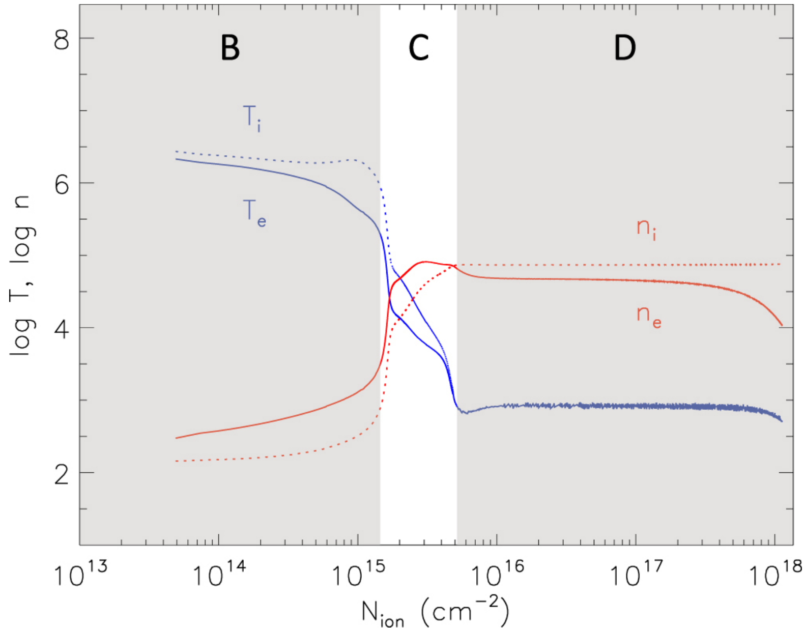
Figure 8. from Probing the Innermost Ejecta Layers in Supernova Remnant Kes 75: Implications for the Supernova Progenitor null 2019 APJL 878 L19 doi:10.3847/2041-8213/ab237c https://dx.doi.org/10.3847/2041-8213/ab237c © 2019. The American Astronomical Society. All rights reserved.
