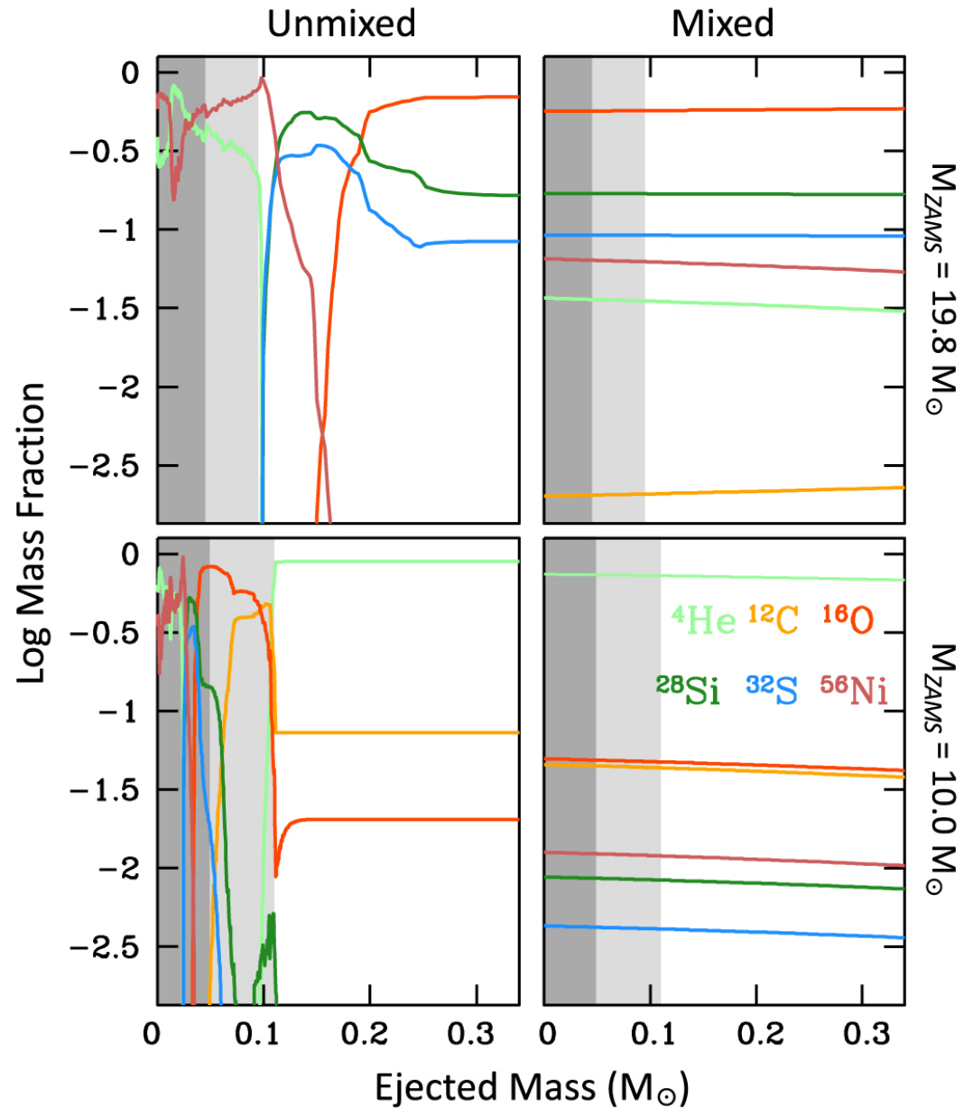
Figure 7. from Probing the Innermost Ejecta Layers in Supernova Remnant Kes 75: Implications for the Supernova Progenitor null 2019 APJL 878 L19 doi:10.3847/2041-8213/ab237c https://dx.doi.org/10.3847/2041-8213/ab237c © 2019. The American Astronomical Society. All rights reserved.
