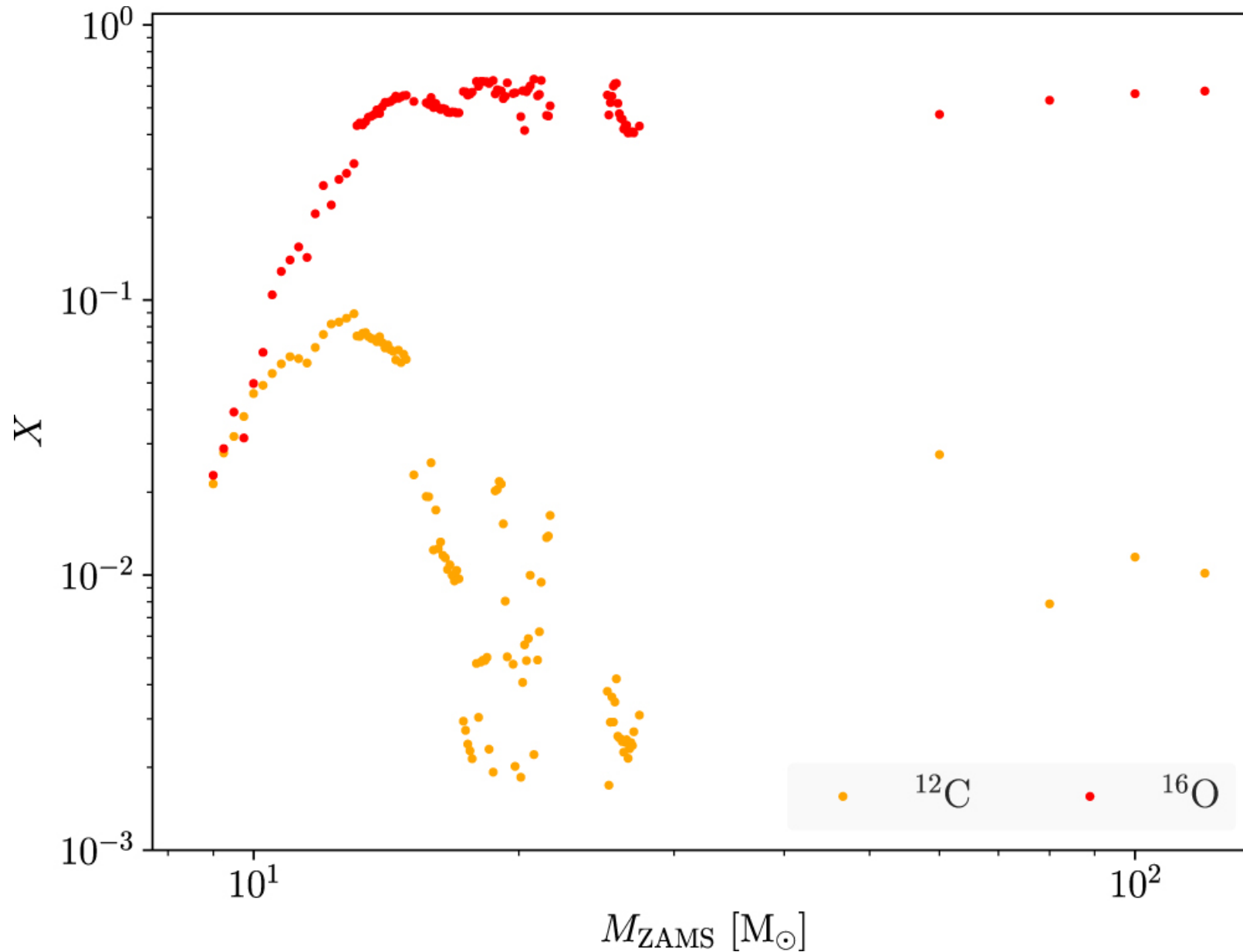
Figure 10. from Probing the Innermost Ejecta Layers in Supernova Remnant Kes 75: Implications for the Supernova Progenitor null 2019 APJL 878 L19 doi:10.3847/2041-8213/ab237c https://dx.doi.org/10.3847/2041-8213/ab237c © 2019. The American Astronomical Society. All rights reserved.
