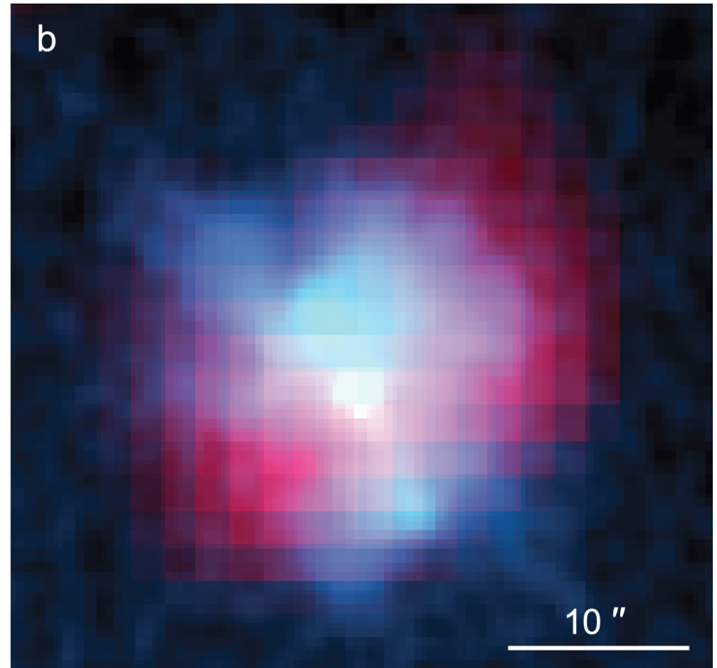
Figure 1. from Probing the Innermost Ejecta Layers in Supernova Remnant Kes 75: Implications for the Supernova Progenitor null 2019 APJL 878 L19 doi:10.3847/2041-8213/ab237c https://dx.doi.org/10.3847/2041-8213/ab237c © 2019. The American Astronomical Society. All rights reserved.
