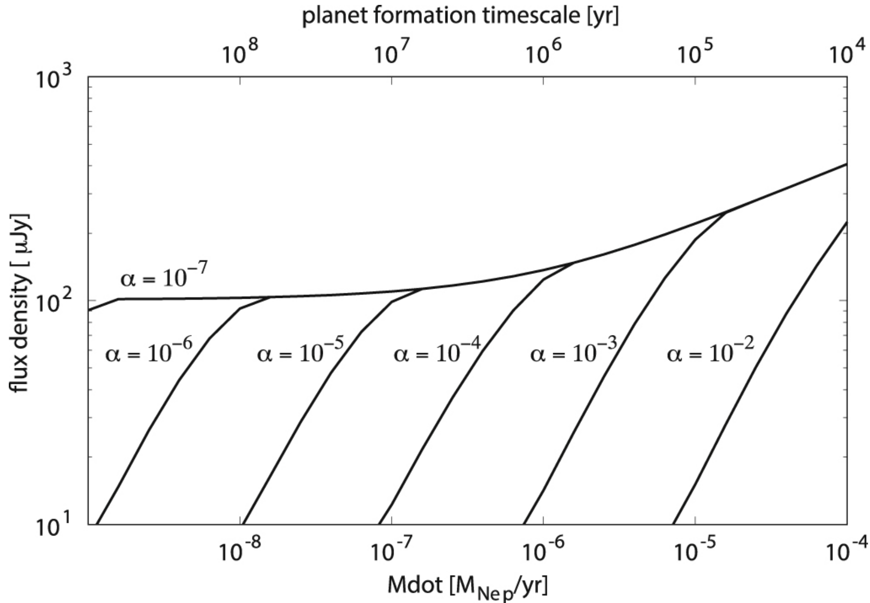
Figure 5. from Discovery of An au-scale Excess in Millimeter Emission from the Protoplanetary Disk around TW Hya null 2019 APJL 878 L8 doi:10.3847/2041-8213/ab224c https://dx.doi.org/10.3847/2041-8213/ab224c © 2019. The American Astronomical Society. All rights reserved.
