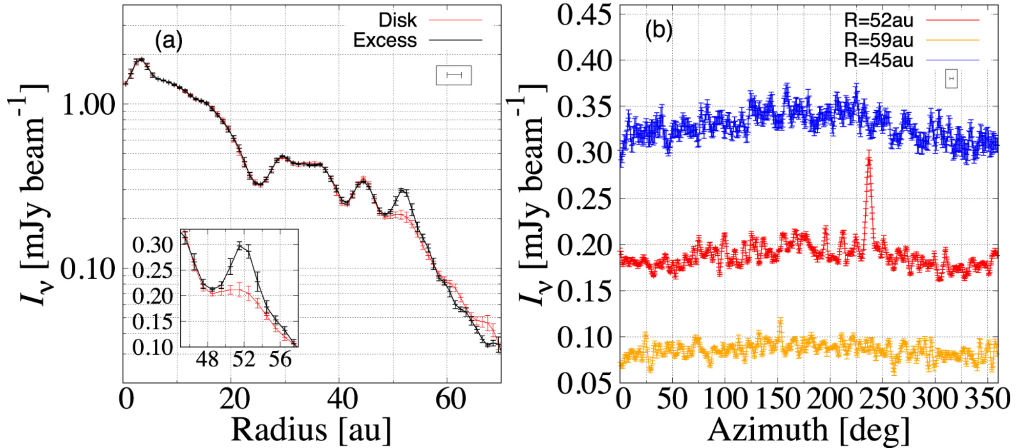
Figure 2. from Discovery of An au-scale Excess in Millimeter Emission from the Protoplanetary Disk around TW Hya null 2019 APJL 878 L8 doi:10.3847/2041-8213/ab224c https://dx.doi.org/10.3847/2041-8213/ab224c © 2019. The American Astronomical Society. All rights reserved.
