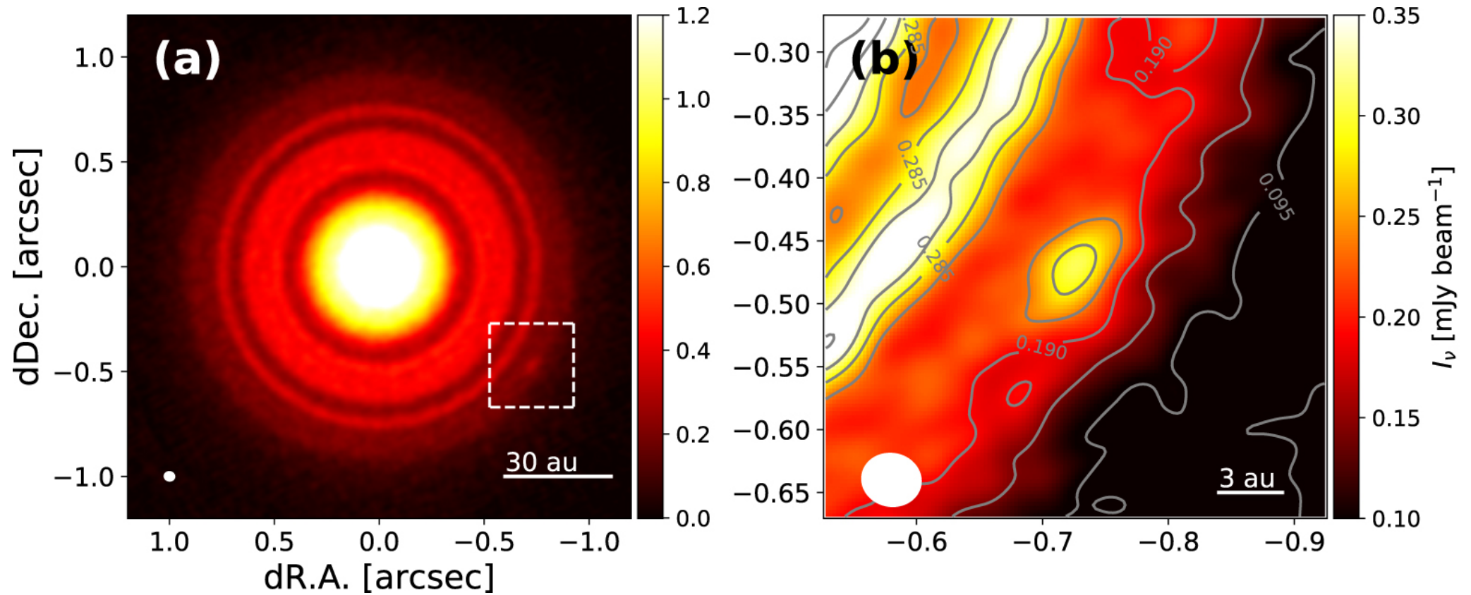
Figure 1. from Discovery of An au-scale Excess in Millimeter Emission from the Protoplanetary Disk around TW Hya null 2019 APJL 878 L8 doi:10.3847/2041-8213/ab224c https://dx.doi.org/10.3847/2041-8213/ab224c © 2019. The American Astronomical Society. All rights reserved.
