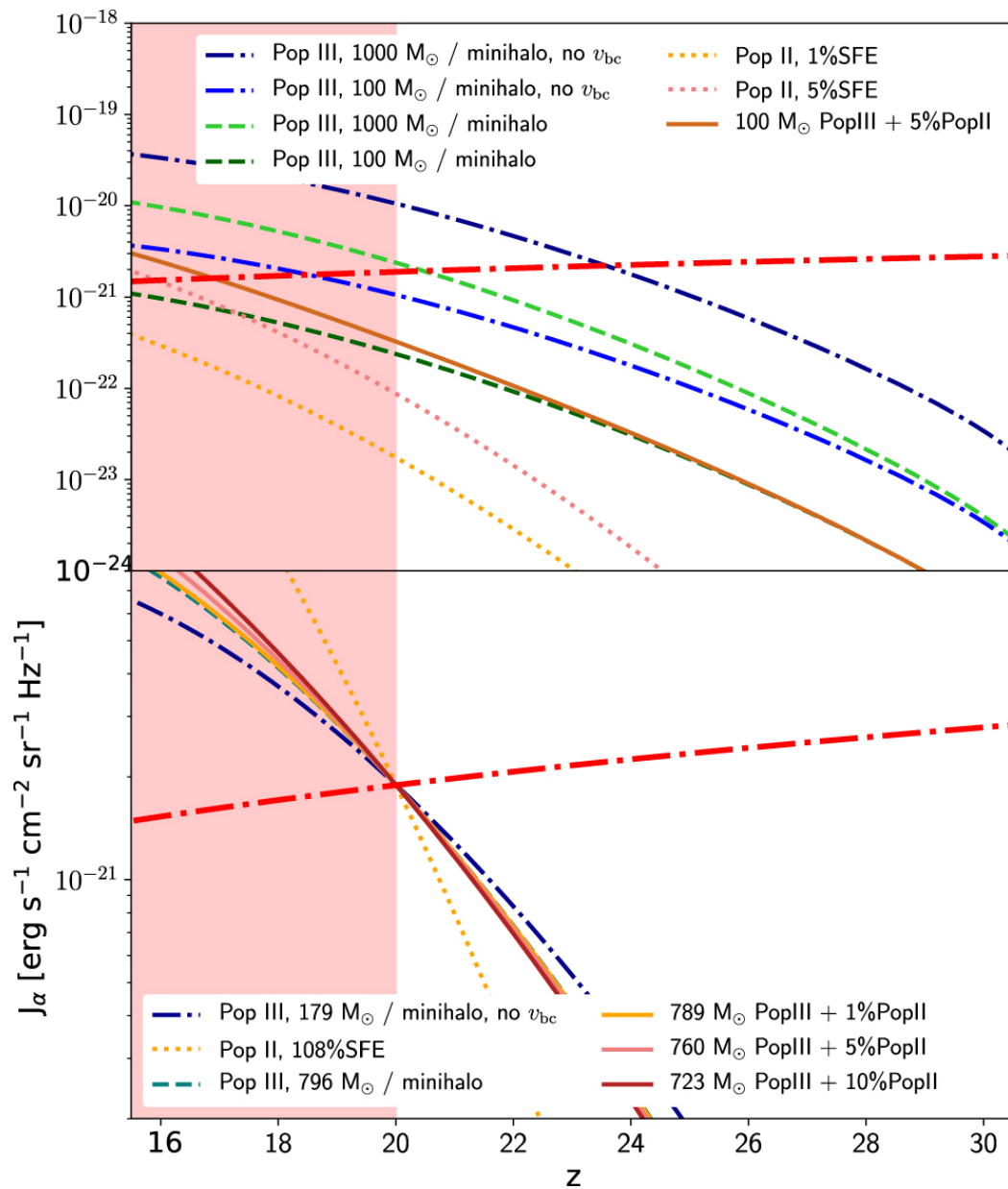
Figure 4. from Constraining First Star Formation with 21 cm Cosmology null 2019 APJL 877 L5 doi:10.3847/2041-8213/ab1e51 https://dx.doi.org/10.3847/2041-8213/ab1e51
