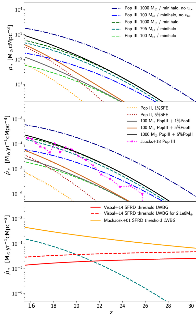
Figure 3. from Constraining First Star Formation with 21 cm Cosmology null 2019 APJL 877 L5 doi:10.3847/2041-8213/ab1e51 https://dx.doi.org/10.3847/2041-8213/ab1e51 © 2019. The American Astronomical Society. All rights reserved.
