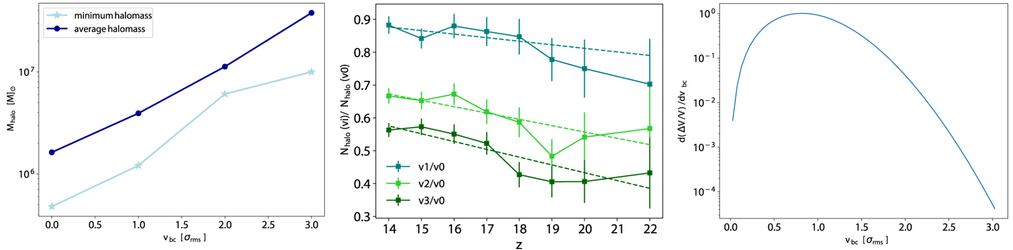
Figure 1. from Constraining First Star Formation with 21 cm Cosmology null 2019 APJL 877 L5 doi:10.3847/2041-8213/ab1e51 https://dx.doi.org/10.3847/2041-8213/ab1e51 © 2019. The American Astronomical Society. All rights reserved.
