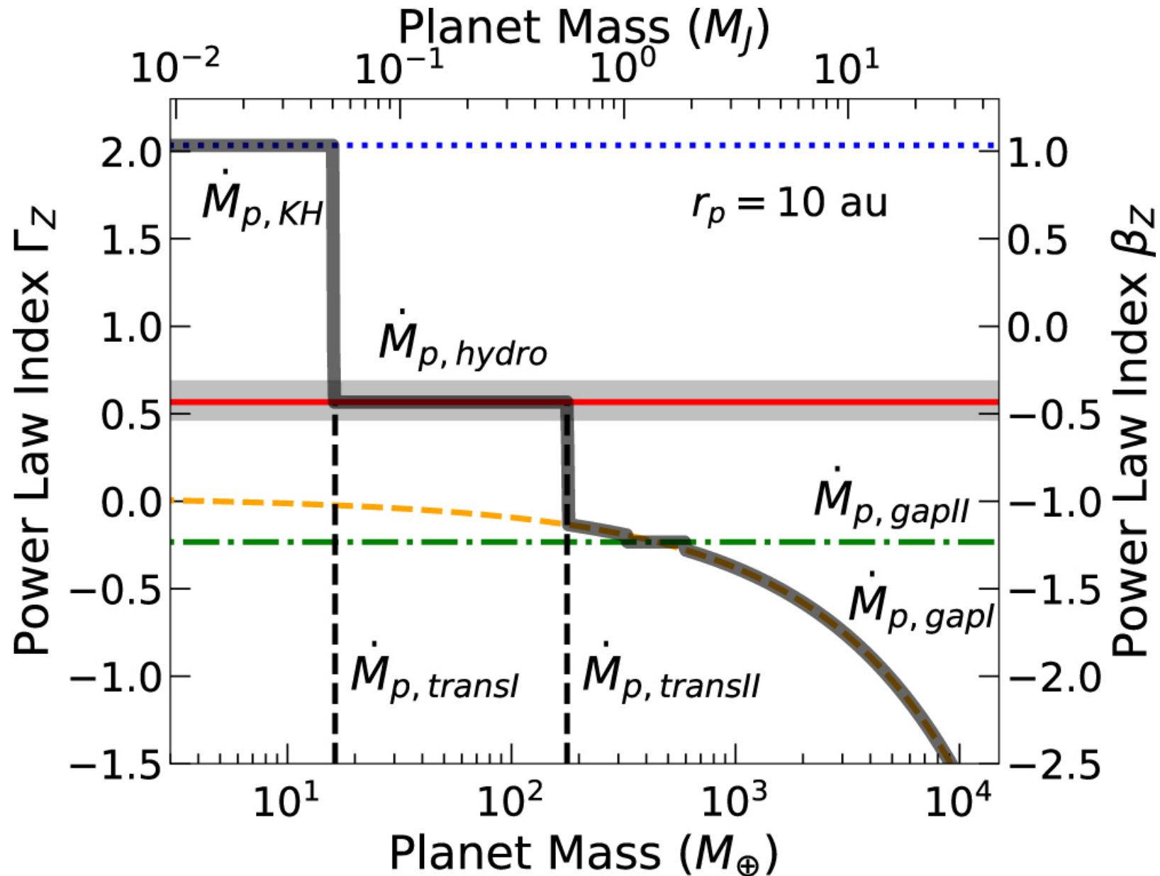
Figure 2. from The Heavy-element Content Trend of Planets: A Tracer of Their Formation Sites null 2019 APJL 876 L32 doi:10.3847/2041-8213/ab1b5a https://dx.doi.org/10.3847/2041-8213/ab1b5a © 2019. The American Astronomical Society. All rights reserved.
