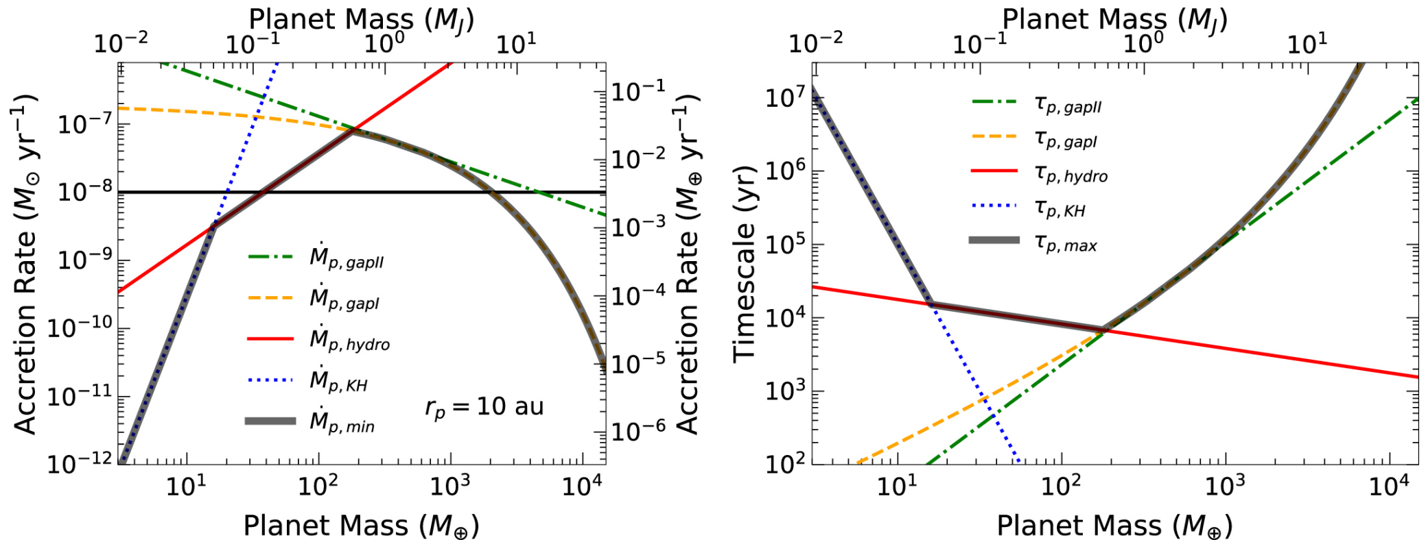
Figure 1. from The Heavy-element Content Trend of Planets: A Tracer of Their Formation Sites null 2019 APJL 876 L32 doi:10.3847/2041-8213/ab1b5a https://dx.doi.org/10.3847/2041-8213/ab1b5a © 2019. The American Astronomical Society. All rights reserved.
