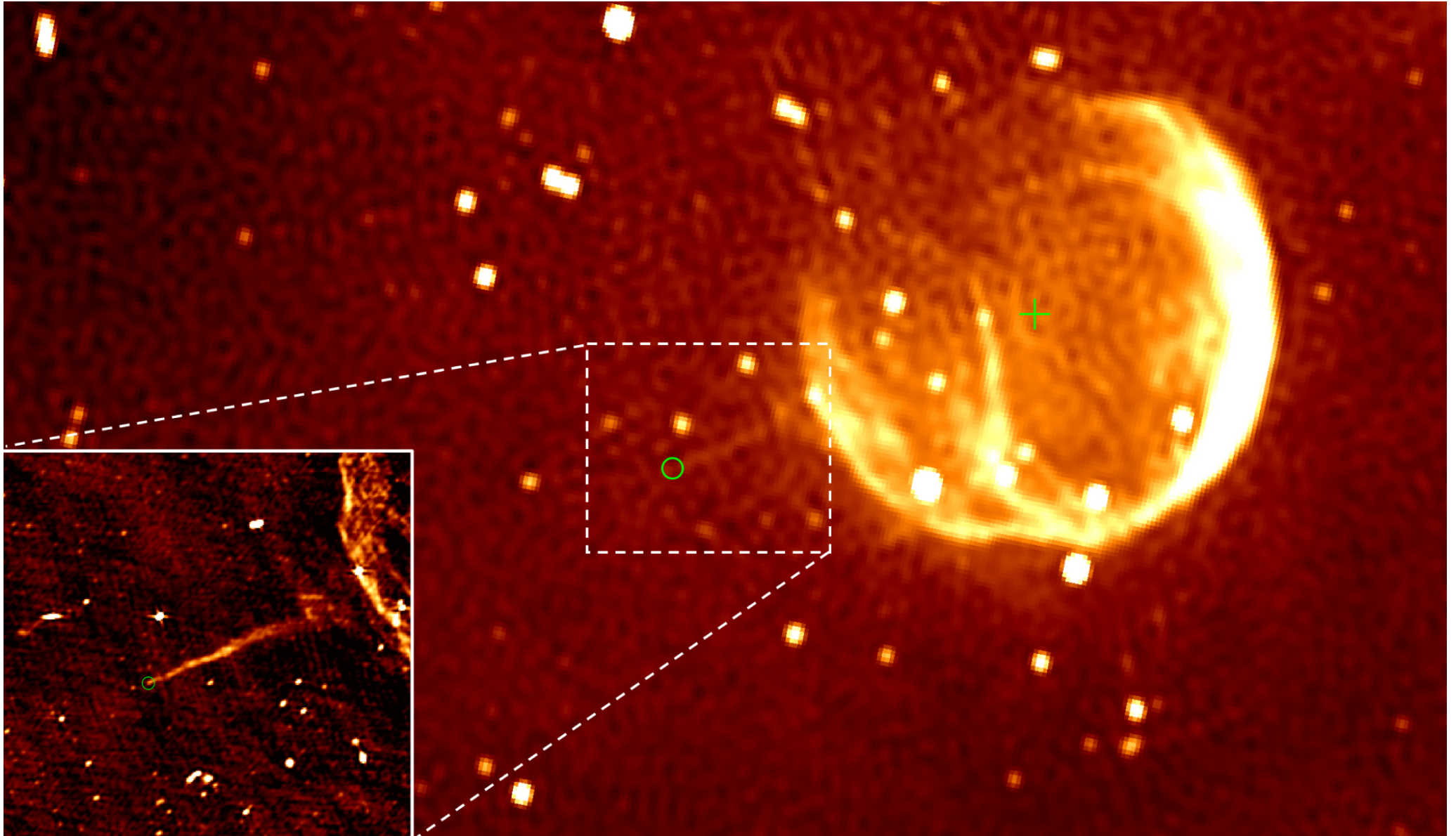
Figure 4. from The Tail of PSR J0002+6216 and the Supernova Remnant CTB 1 null 2019 APJL 876 L17 doi:10.3847/2041-8213/ab18f7 https://dx.doi.org/10.3847/2041-8213/ab18f7 © 2019. The American Astronomical Society. All rights reserved.
