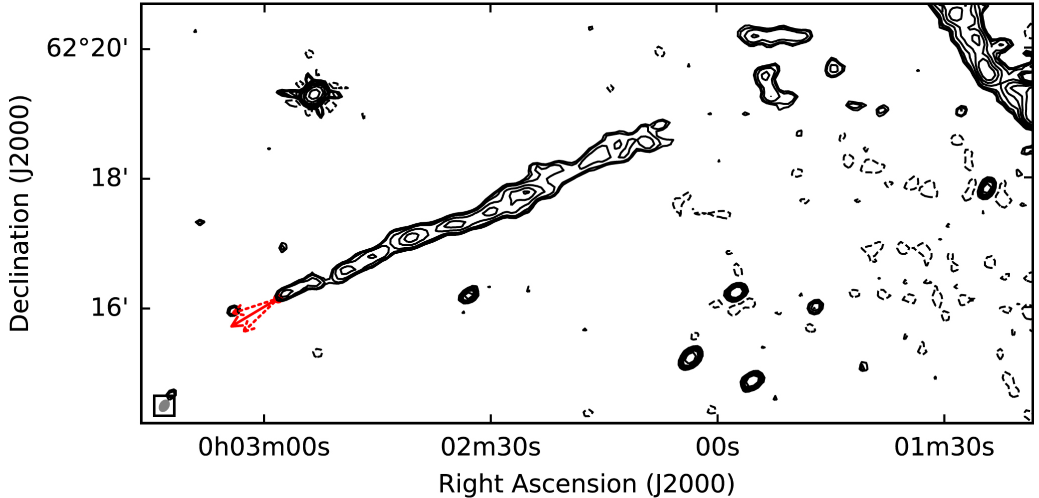
Figure 3. from The Tail of PSR J0002+6216 and the Supernova Remnant CTB 1 null 2019 APJL 876 L17 doi:10.3847/2041-8213/ab18f7 https://dx.doi.org/10.3847/2041-8213/ab18f7 © 2019. The American Astronomical Society. All rights reserved.
