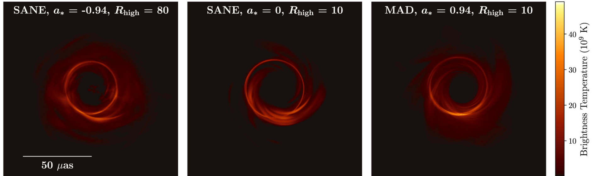
Figure 4. from First M87 Event Horizon Telescope Results. I. The Shadow of the Supermassive Black Hole null 2019 APJL 875 L1 doi:10.3847/2041-8213/ab0ec7 https://dx.doi.org/10.3847/2041-8213/ab0ec7 © 2019. The American Astronomical Society.
