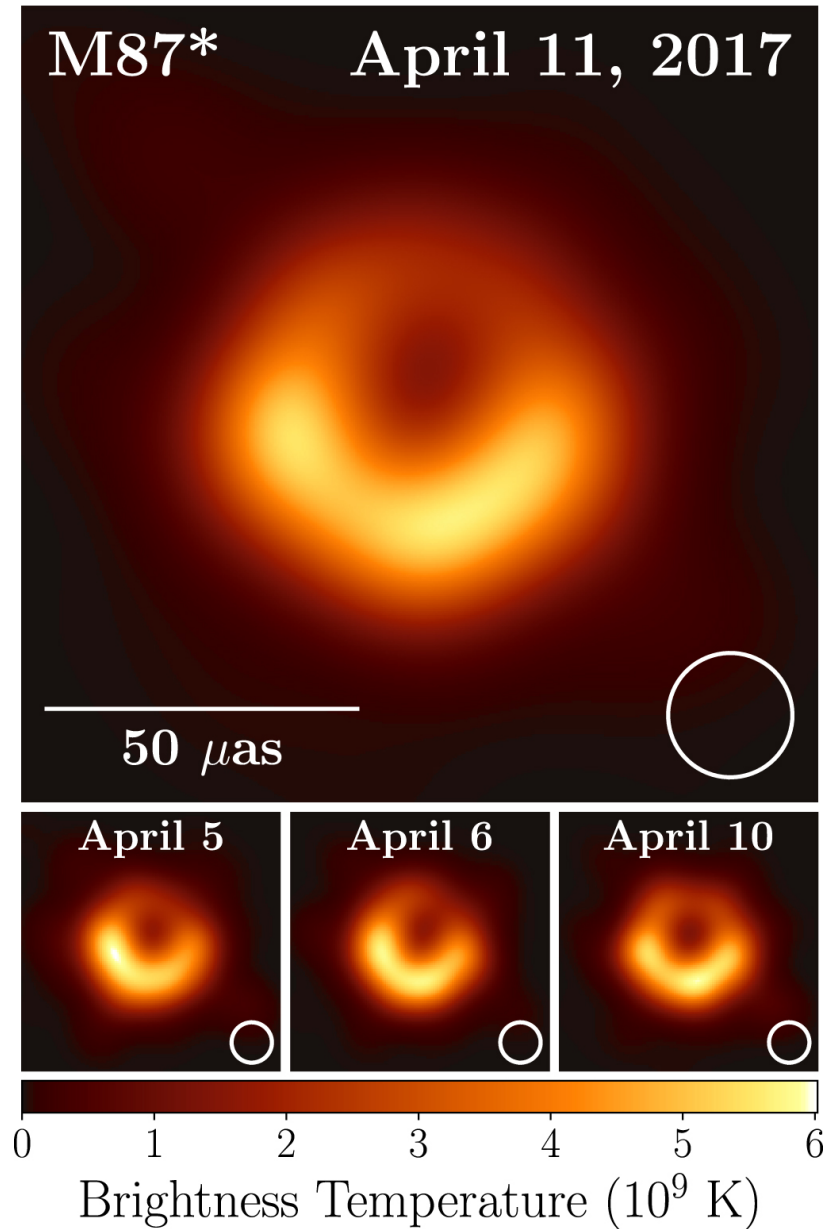
Figure 3. from First M87 Event Horizon Telescope Results. I. The Shadow of the Supermassive Black Hole null 2019 APJL 875 L1 doi:10.3847/2041-8213/ab0ec7 https://dx.doi.org/10.3847/2041-8213/ab0ec7 © 2019. The American Astronomical Society.
