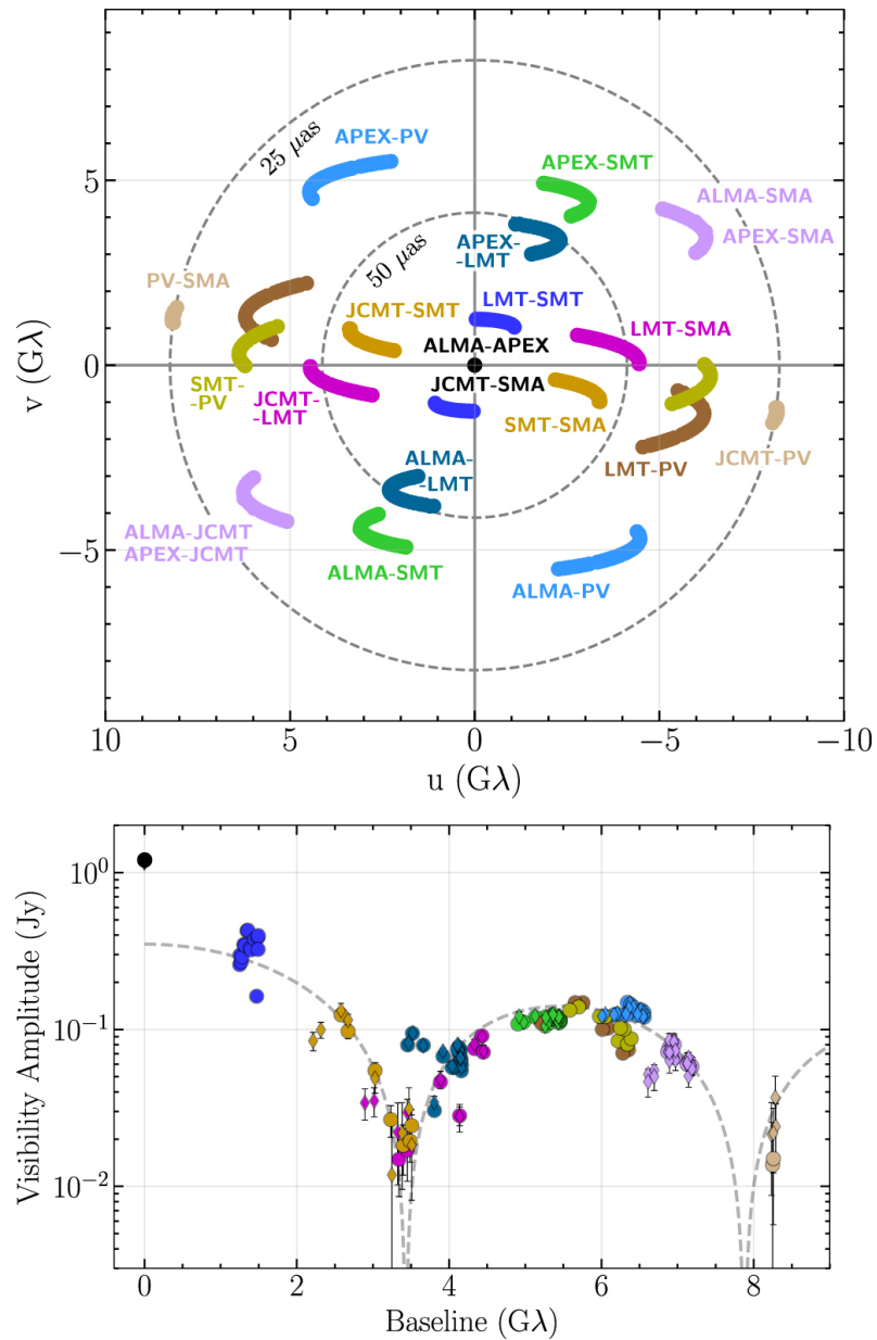
Figure 2. from First M87 Event Horizon Telescope Results. I. The Shadow of the Supermassive Black Hole null 2019 APJL 875 L1 doi:10.3847/2041-8213/ab0ec7 https://dx.doi.org/10.3847/2041-8213/ab0ec7 © 2019. The American Astronomical Society.
