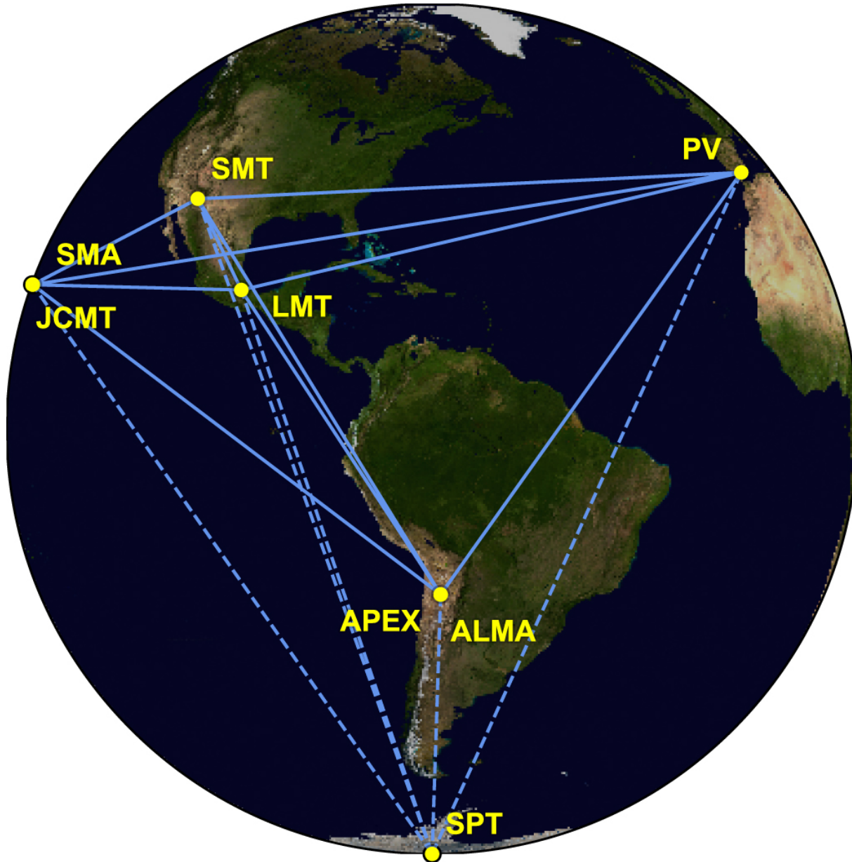
Figure 1. from First M87 Event Horizon Telescope Results. I. The Shadow of the Supermassive Black Hole null 2019 APJL 875 L1 doi:10.3847/2041-8213/ab0ec7 https://dx.doi.org/10.3847/2041-8213/ab0ec7 © 2019. The American Astronomical Society.
