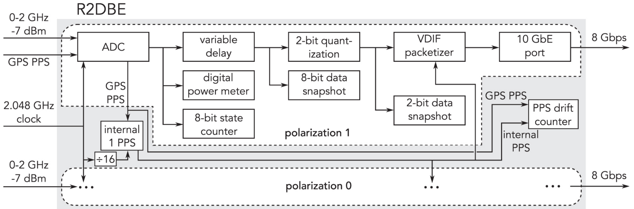
Figure 7. from First M87 Event Horizon Telescope Results. II. Array and Instrumentation null 2019 APJL 875 L2 doi:10.3847/2041-8213/ab0c96 https://dx.doi.org/10.3847/2041-8213/ab0c96 © 2019. The American Astronomical Society.
