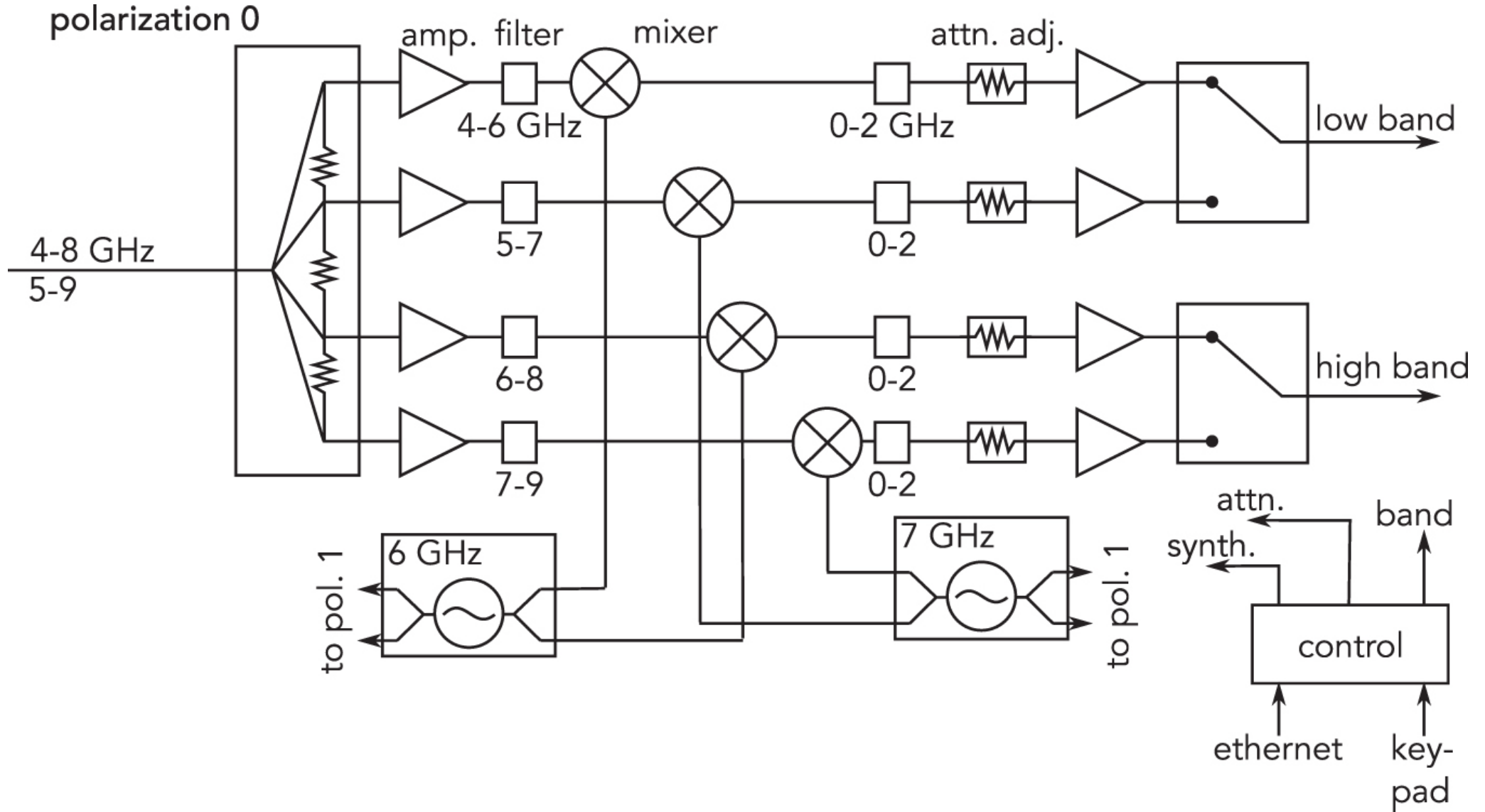
Figure 6. from First M87 Event Horizon Telescope Results. II. Array and Instrumentation null 2019 APJL 875 L2 doi:10.3847/2041-8213/ab0c96 https://dx.doi.org/10.3847/2041-8213/ab0c96 © 2019. The American Astronomical Society.
