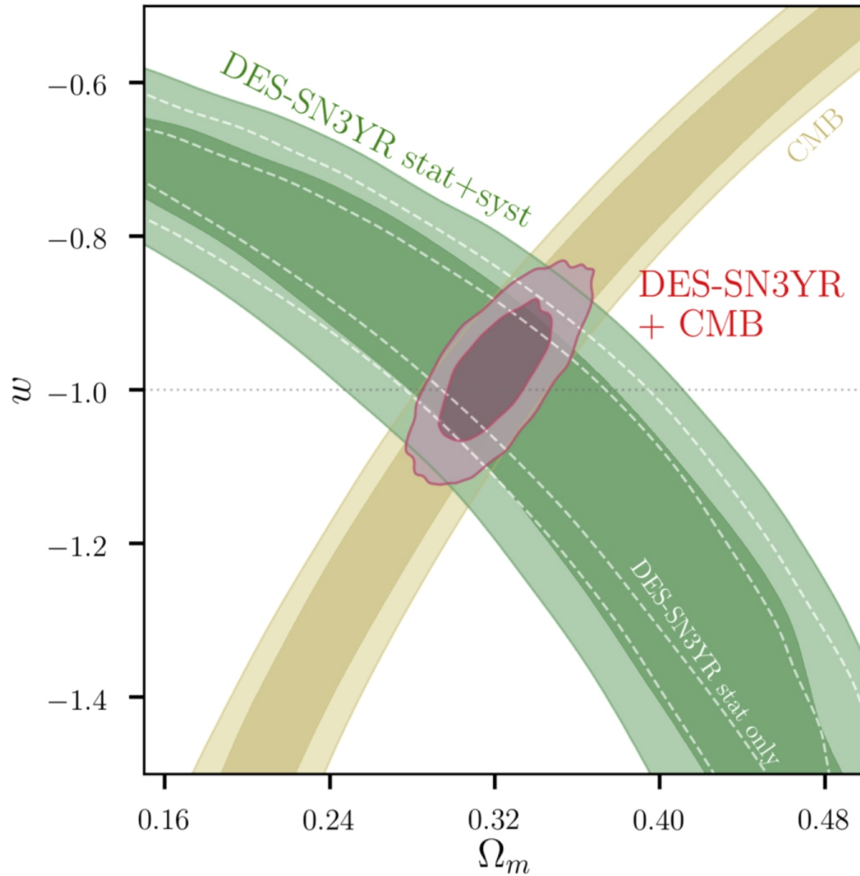
Figure 3. from First Cosmology Results using Type Ia Supernovae from the Dark Energy Survey: Constraints on Cosmological Parameters null 2019 APJL 872 L30 doi:10.3847/2041-8213/ab04fa https://dx.doi.org/10.3847/2041-8213/ab04fa © 2019. The American Astronomical Society. All rights reserved.
