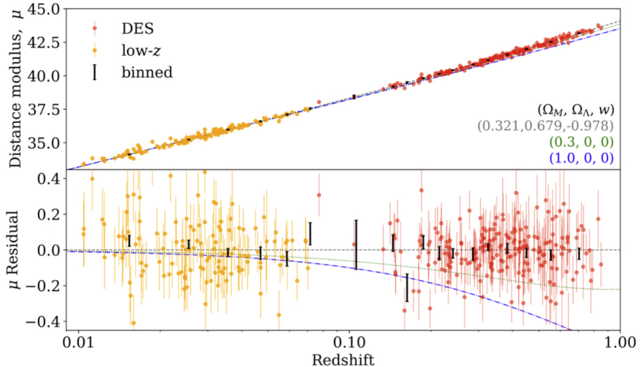
Figure 1. from First Cosmology Results using Type Ia Supernovae from the Dark Energy Survey: Constraints on Cosmological Parameters null 2019 APJL 872 L30 doi:10.3847/2041-8213/ab04fa https://dx.doi.org/10.3847/2041-8213/ab04fa © 2019. The American Astronomical Society. All rights reserved.
