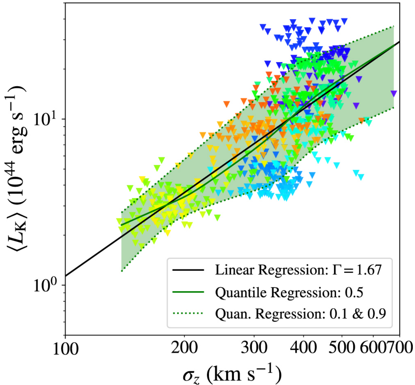
Figure 4. from Using H Filaments to Probe Active Galactic Nuclei Feedback in Galaxy Clusters null 2019 APJL 872 L11 doi:10.3847/2041-8213/ab0375 https://dx.doi.org/10.3847/2041-8213/ab0375 © 2019. The American Astronomical Society. All rights reserved.
