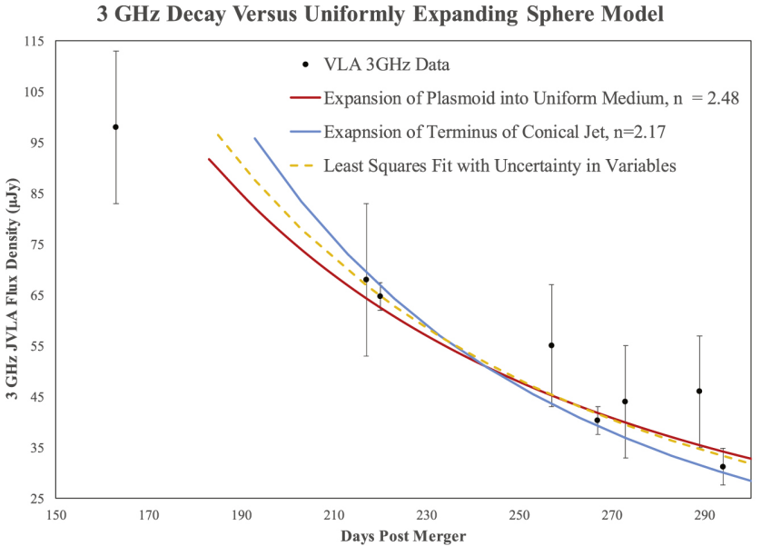
Figure 5. from Discrete and Continuous Ejection Models of the Radio Source Associated with GW170817 null 2019 APJL 871 L34 doi:10.3847/2041-8213/ab01e0 https://dx.doi.org/10.3847/2041-8213/ab01e0 © 2019. The American Astronomical Society. All rights reserved.
