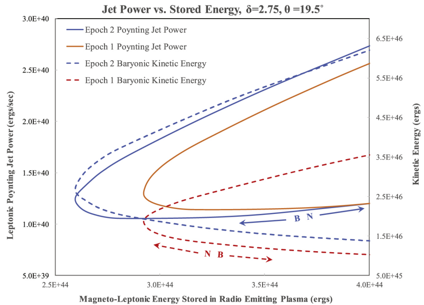
Figure 3. from Discrete and Continuous Ejection Models of the Radio Source Associated with GW170817 null 2019 APJL 871 L34 doi:10.3847/2041-8213/ab01e0 https://dx.doi.org/10.3847/2041-8213/ab01e0
