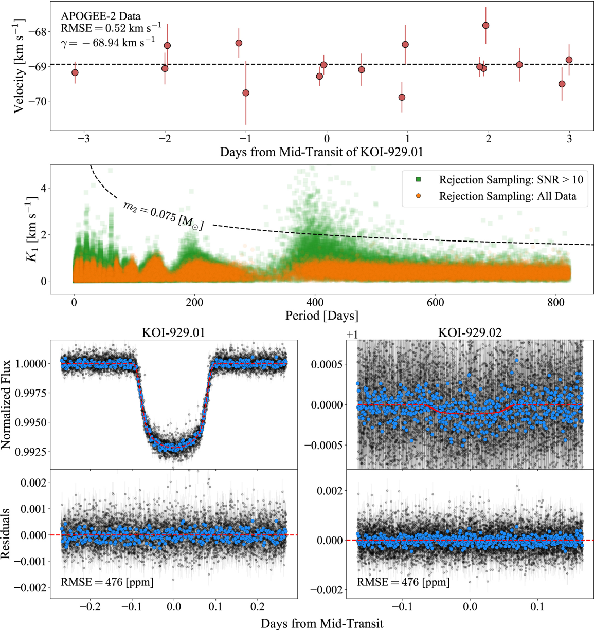
Figure 2. from Kepler-730: A Hot Jupiter System with a Close-in, Transiting, Earth-sized Planet null 2019 APJL 870 L17 doi:10.3847/2041-8213/aafa1e https://dx.doi.org/10.3847/2041-8213/aafa1e © 2019. The American Astronomical Society. All rights reserved.
