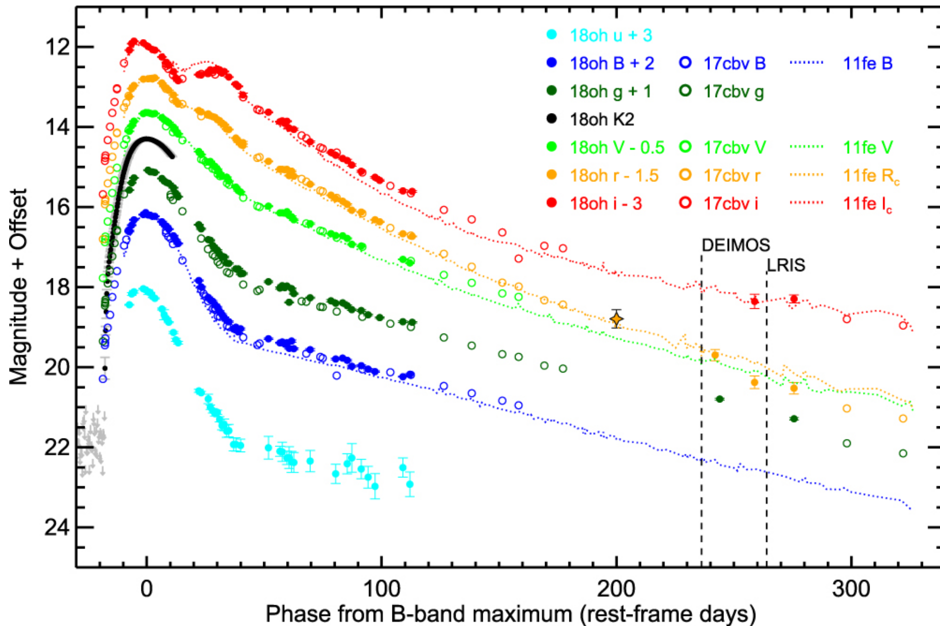
Figure 2. from Nebular Spectroscopy of Kepler's Brightest Supernova null 2019 APJL 870 L14 doi:10.3847/2041-8213/aaf9b1 https://dx.doi.org/10.3847/2041-8213/aaf9b1 © 2019. The American Astronomical Society. All rights reserved.
