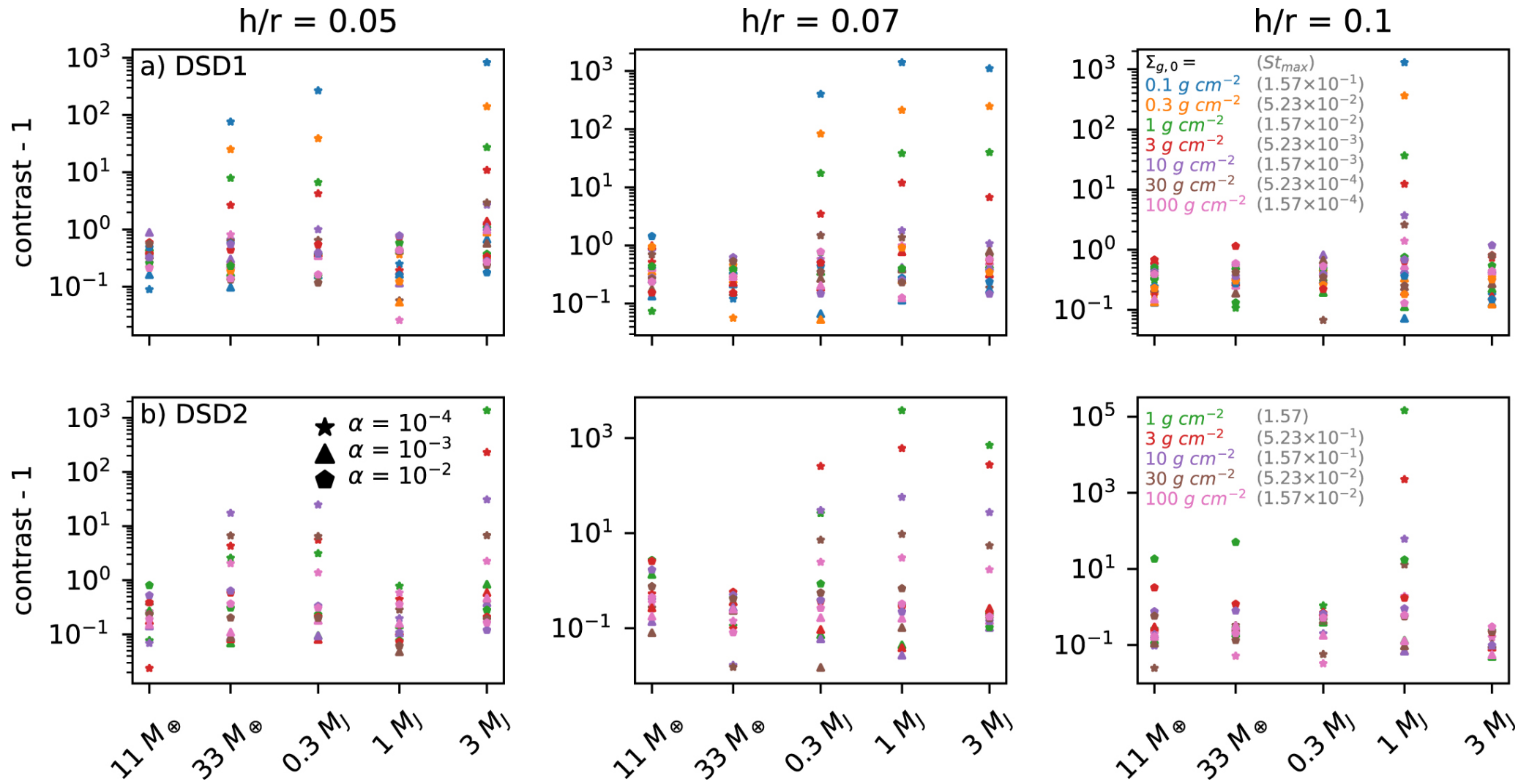
Figure 9. from The Disk Substructures at High Angular Resolution Project (DSHARP). VII. The Planet–Disk Interactions Interpretation null 2018 APJL 869 L47 doi:10.3847/2041-8213/aaf744 https://dx.doi.org/10.3847/2041-8213/aaf744 © 2018. The American Astronomical Society. All rights reserved.
