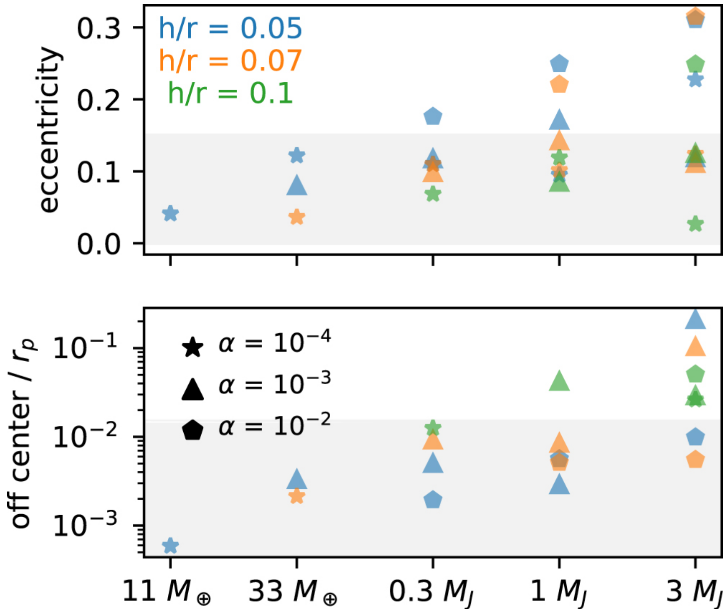
Figure 8. from The Disk Substructures at High Angular Resolution Project (DSHARP). VII. The Planet–Disk Interactions Interpretation null 2018 APJL 869 L47 doi:10.3847/2041-8213/aaf744 https://dx.doi.org/10.3847/2041-8213/aaf744 © 2018. The American Astronomical Society. All rights reserved.
