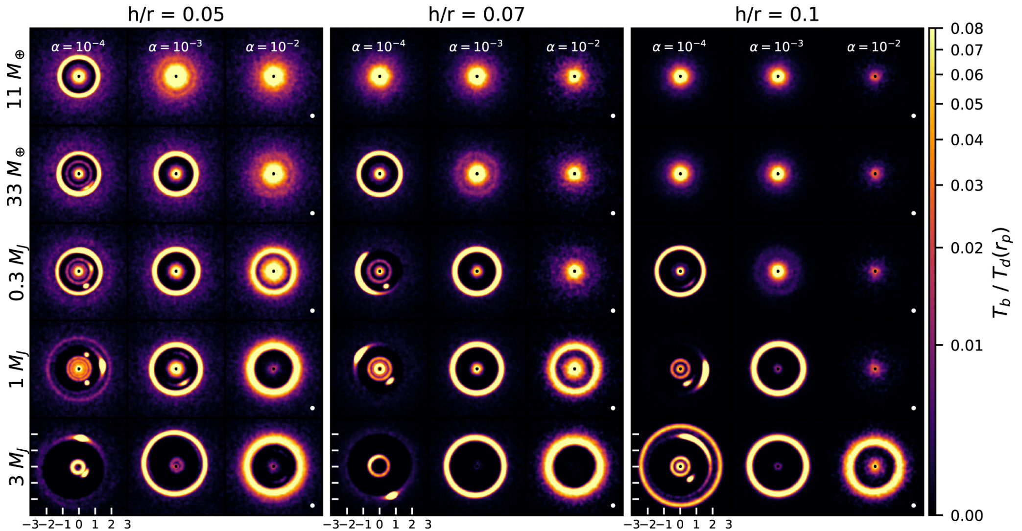
Figure 7. from The Disk Substructures at High Angular Resolution Project (DSHARP). VII. The Planet–Disk Interactions Interpretation null 2018 APJL 869 L47 doi:10.3847/2041-8213/aaf744 https://dx.doi.org/10.3847/2041-8213/aaf744 © 2018. The American Astronomical Society. All rights reserved.
