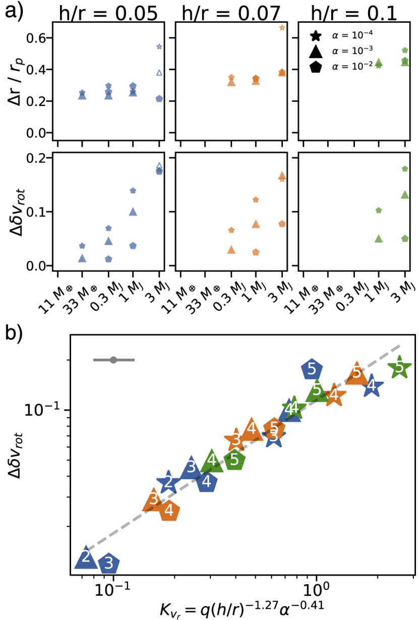
Figure 5. from The Disk Substructures at High Angular Resolution Project (DSHARP). VII. The Planet–Disk Interactions Interpretation null 2018 APJL 869 L47 doi:10.3847/2041-8213/aaf744 https://dx.doi.org/10.3847/2041-8213/aaf744 © 2018. The American Astronomical Society. All rights reserved.
