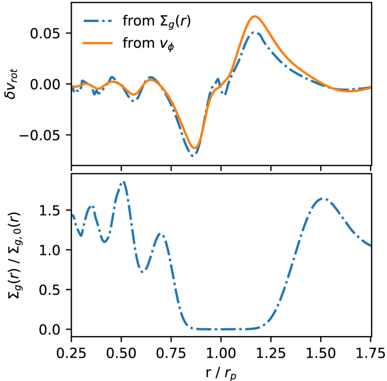
Figure 3. from The Disk Substructures at High Angular Resolution Project (DSHARP). VII. The Planet–Disk Interactions Interpretation null 2018 APJL 869 L47 doi:10.3847/2041-8213/aaf744 https://dx.doi.org/10.3847/2041-8213/aaf744 © 2018. The American Astronomical Society. All rights reserved.
