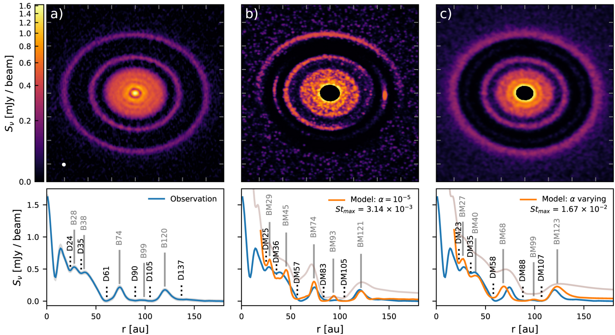
Figure 19. from The Disk Substructures at High Angular Resolution Project (DSHARP). VII. The Planet–Disk Interactions Interpretation null 2018 APJL 869 L47 doi:10.3847/2041-8213/aaf744 https://dx.doi.org/10.3847/2041-8213/aaf744 © 2018. The American Astronomical Society. All rights reserved.
