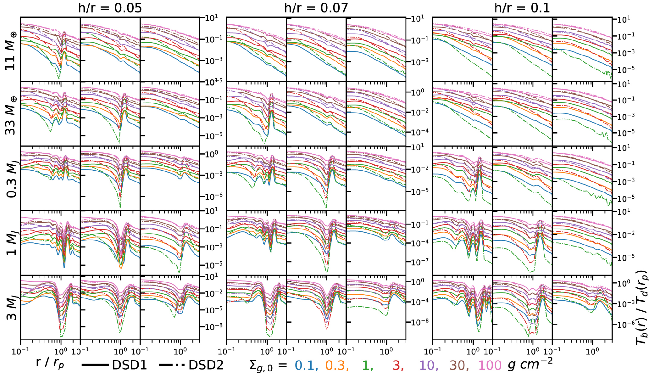
Figure 10. from The Disk Substructures at High Angular Resolution Project (DSHARP). VII. The Planet–Disk Interactions Interpretation null 2018 APJL 869 L47 doi:10.3847/2041-8213/aaf744 https://dx.doi.org/10.3847/2041-8213/aaf744 © 2018. The American Astronomical Society. All rights reserved.
