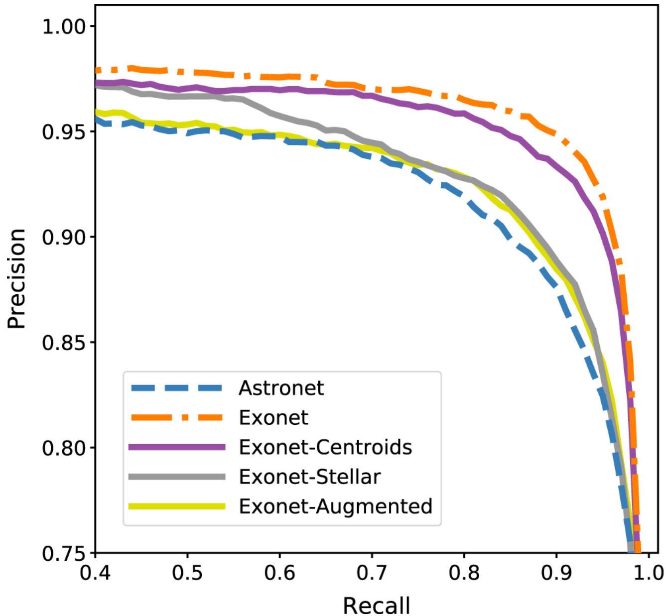
Figure 3. from Scientific Domain Knowledge Improves Exoplanet Transit Classification with Deep Learning null 2018 APJL 869 L7 doi:10.3847/2041-8213/aaf23b https://dx.doi.org/10.3847/2041-8213/aaf23b © 2018. The American Astronomical Society. All rights reserved.
