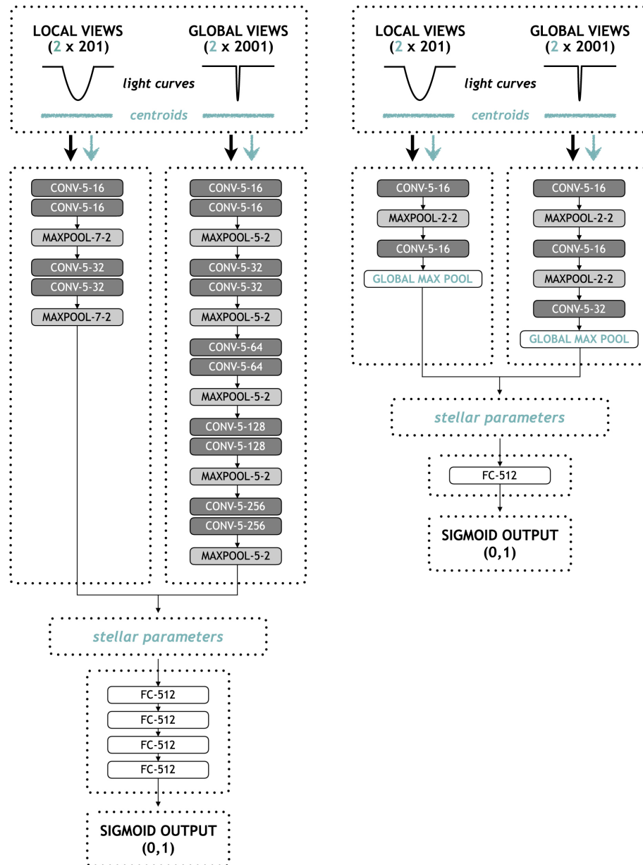
Figure 2. from Scientific Domain Knowledge Improves Exoplanet Transit Classification with Deep Learning null 2018 APJL 869 L7 doi:10.3847/2041-8213/aaf23b https://dx.doi.org/10.3847/2041-8213/aaf23b © 2018. The American Astronomical Society. All rights reserved.
