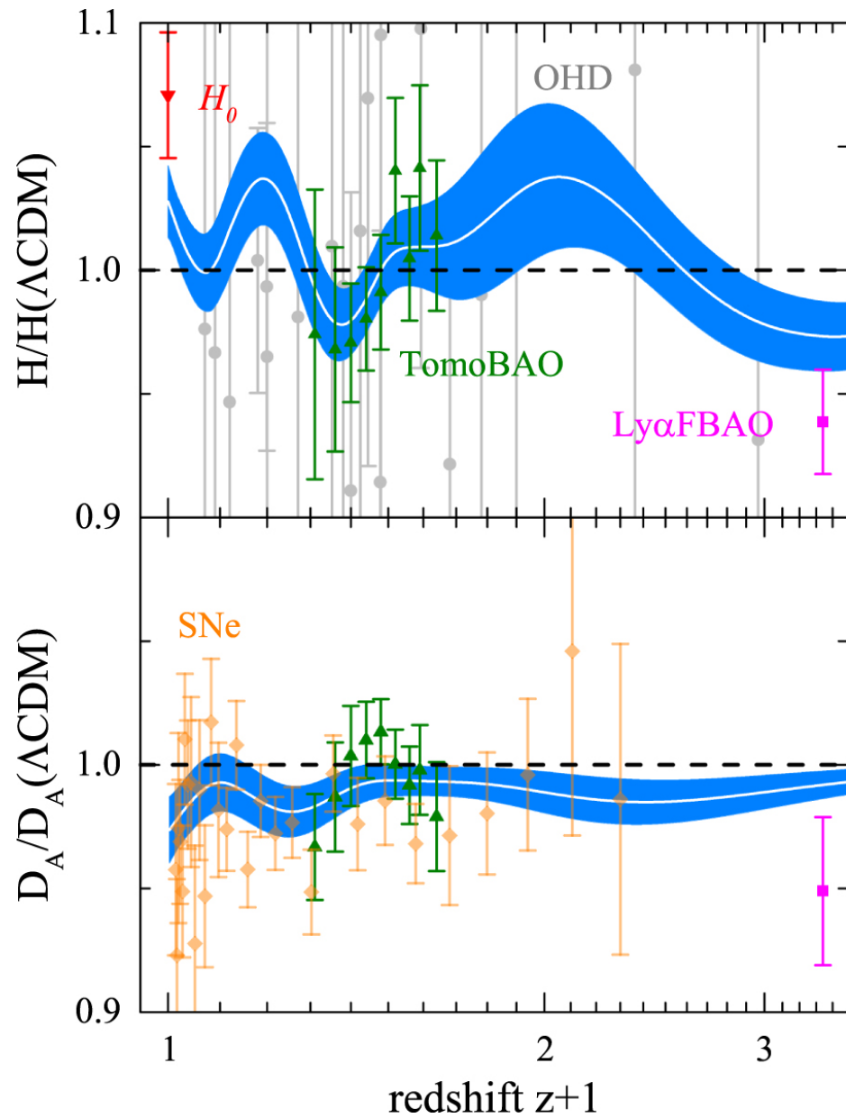
Figure 2. from Evolution of Dark Energy Reconstructed from the Latest Observations null 2018 APJL 869 L8 doi:10.3847/2041-8213/aaf238 https://dx.doi.org/10.3847/2041-8213/aaf238 © 2018. The American Astronomical Society. All rights reserved.
