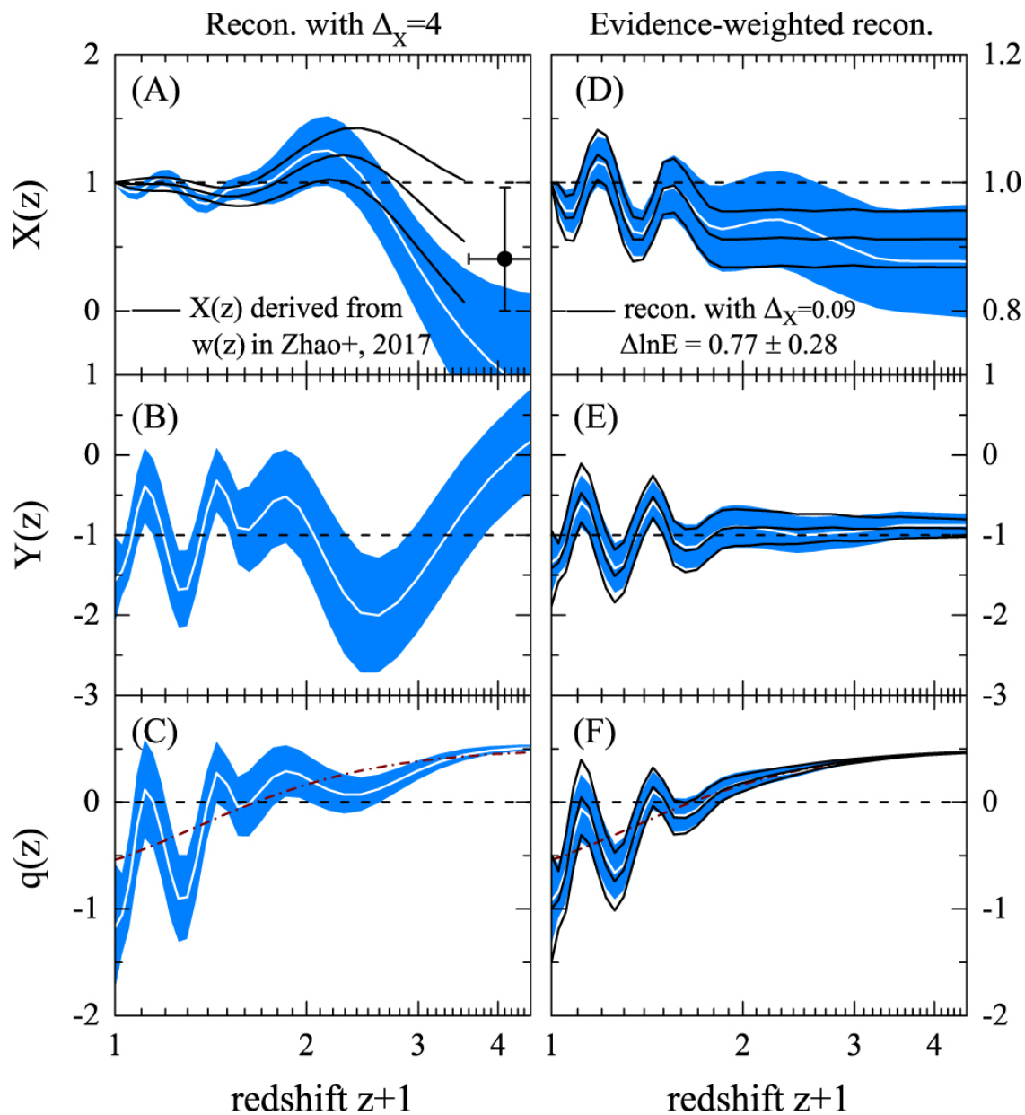
Figure 1. from Evolution of Dark Energy Reconstructed from the Latest Observations null 2018 APJL 869 L8 doi:10.3847/2041-8213/aaf238 https://dx.doi.org/10.3847/2041-8213/aaf238 © 2018. The American Astronomical Society. All rights reserved.
