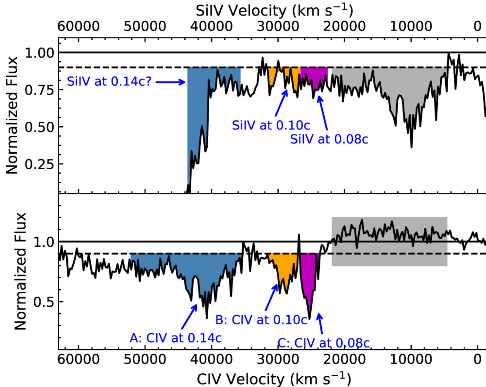
Figure 4. from The Discovery of a Luminous Broad Absorption Line Quasar at a Redshift of 7.02 null 2018 APJL 869 L9 doi:10.3847/2041-8213/aaf1d2 https://dx.doi.org/10.3847/2041-8213/aaf1d2 © 2018. The American Astronomical Society. All rights reserved.
