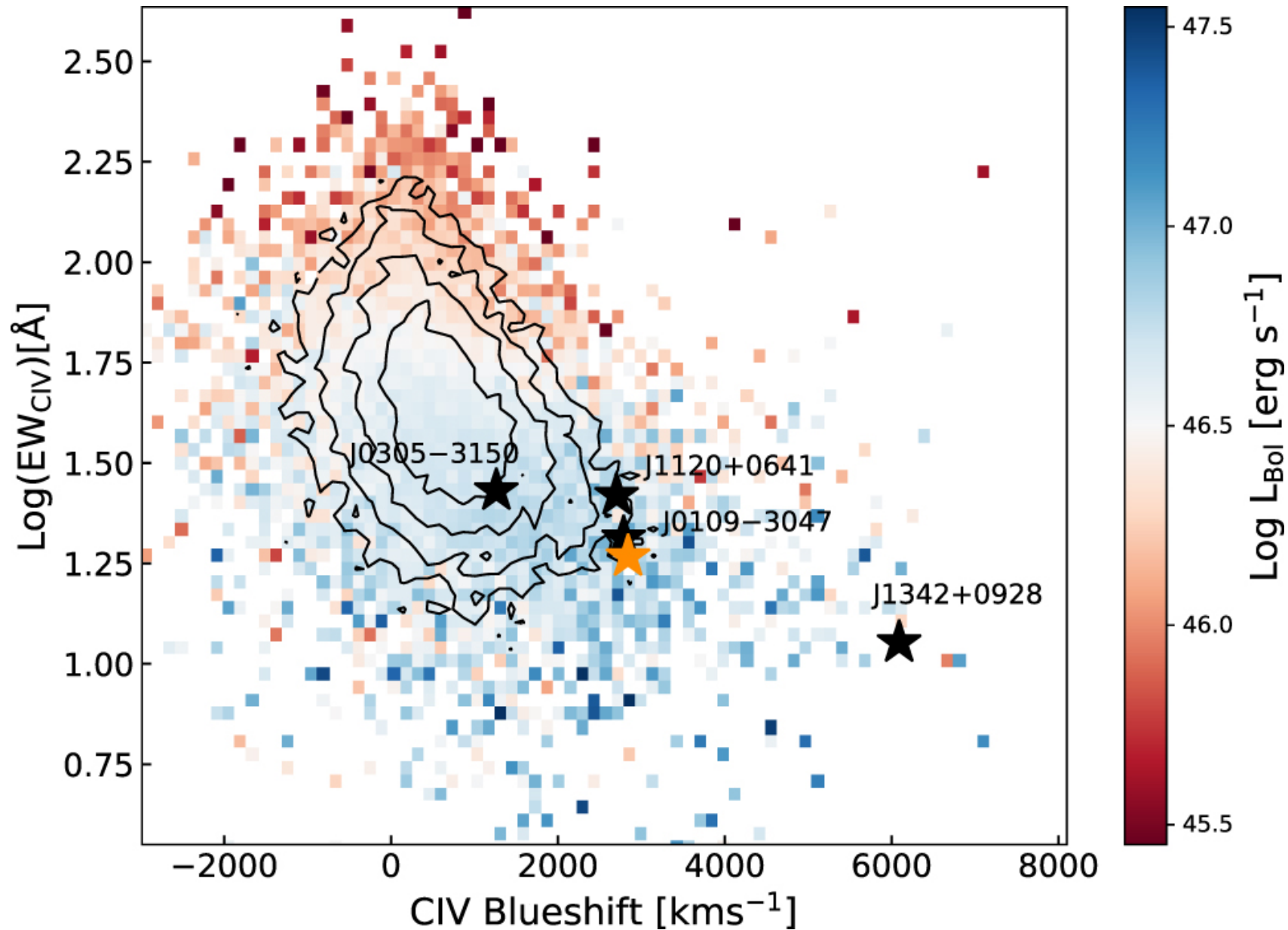
Figure 3. from The Discovery of a Luminous Broad Absorption Line Quasar at a Redshift of 7.02 null 2018 APJL 869 L9 doi:10.3847/2041-8213/aaf1d2 https://dx.doi.org/10.3847/2041-8213/aaf1d2 © 2018. The American Astronomical Society. All rights reserved.
