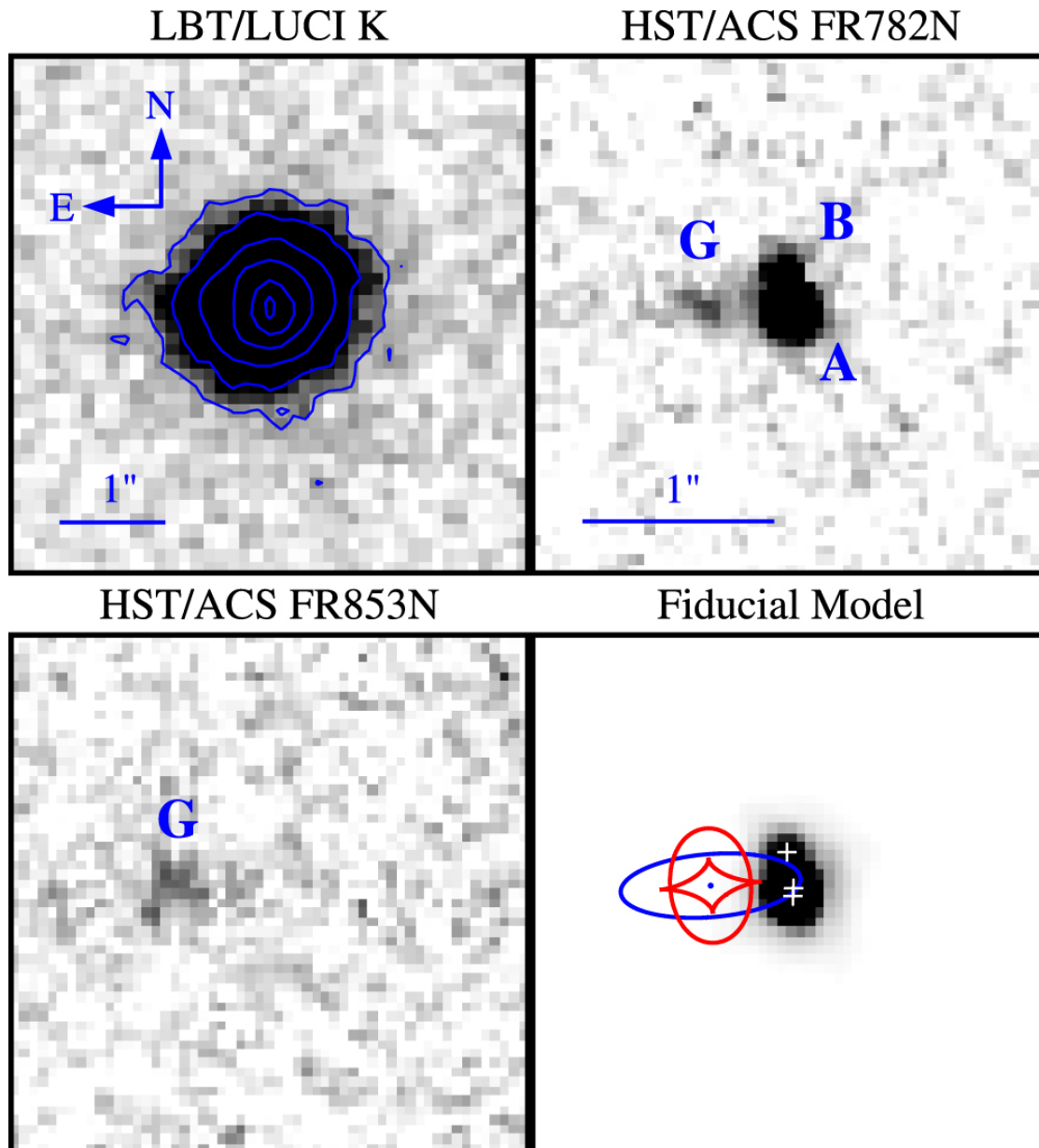
Figure 3. from The Discovery of a Gravitationally Lensed Quasar at z = 6.51 null 2019 APJL 870 L11 doi:10.3847/2041-8213/aaeffe https://dx.doi.org/10.3847/2041-8213/aaeffe © 2019. The American Astronomical Society. All rights reserved.
