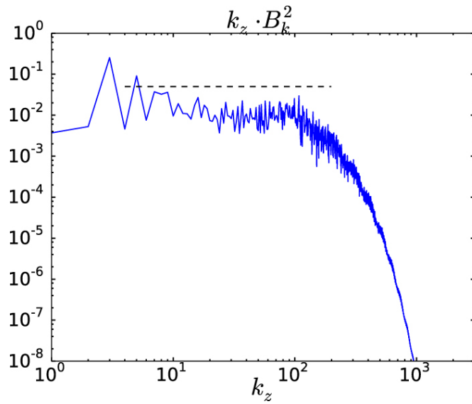
Figure 3. from Nonlinear Firehose Relaxation and Constant-B Field Fluctuations null 2018 APJL 867 L26 doi:10.3847/2041-8213/aaec01 https://dx.doi.org/10.3847/2041-8213/aaec01 © 2018. The American Astronomical Society. All rights reserved.
