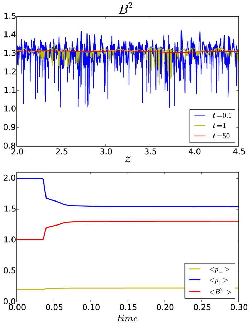
Figure 2. from Nonlinear Firehose Relaxation and Constant-B Field Fluctuations null 2018 APJL 867 L26 doi:10.3847/2041-8213/aaec01 https://dx.doi.org/10.3847/2041-8213/aaec01 © 2018. The American Astronomical Society. All rights reserved.
