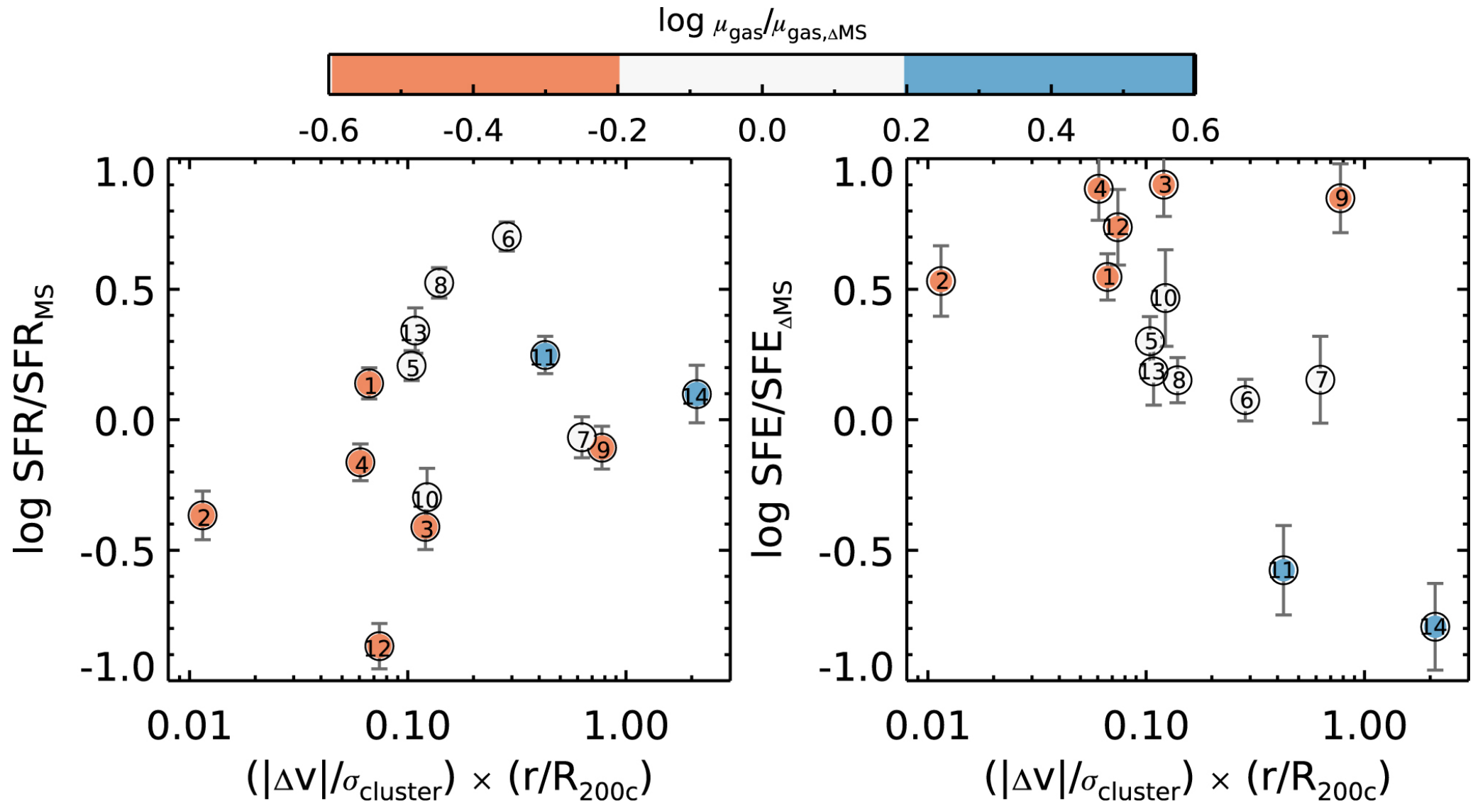
Figure 4. from Revealing the Environmental Dependence of Molecular Gas Content in a Distant X-Ray Cluster at z = 2.51 null 2018 APJL 867 L29 doi:10.3847/2041-8213/aaeb2c https://dx.doi.org/10.3847/2041-8213/aaeb2c © 2018. The American Astronomical Society. All rights reserved.
