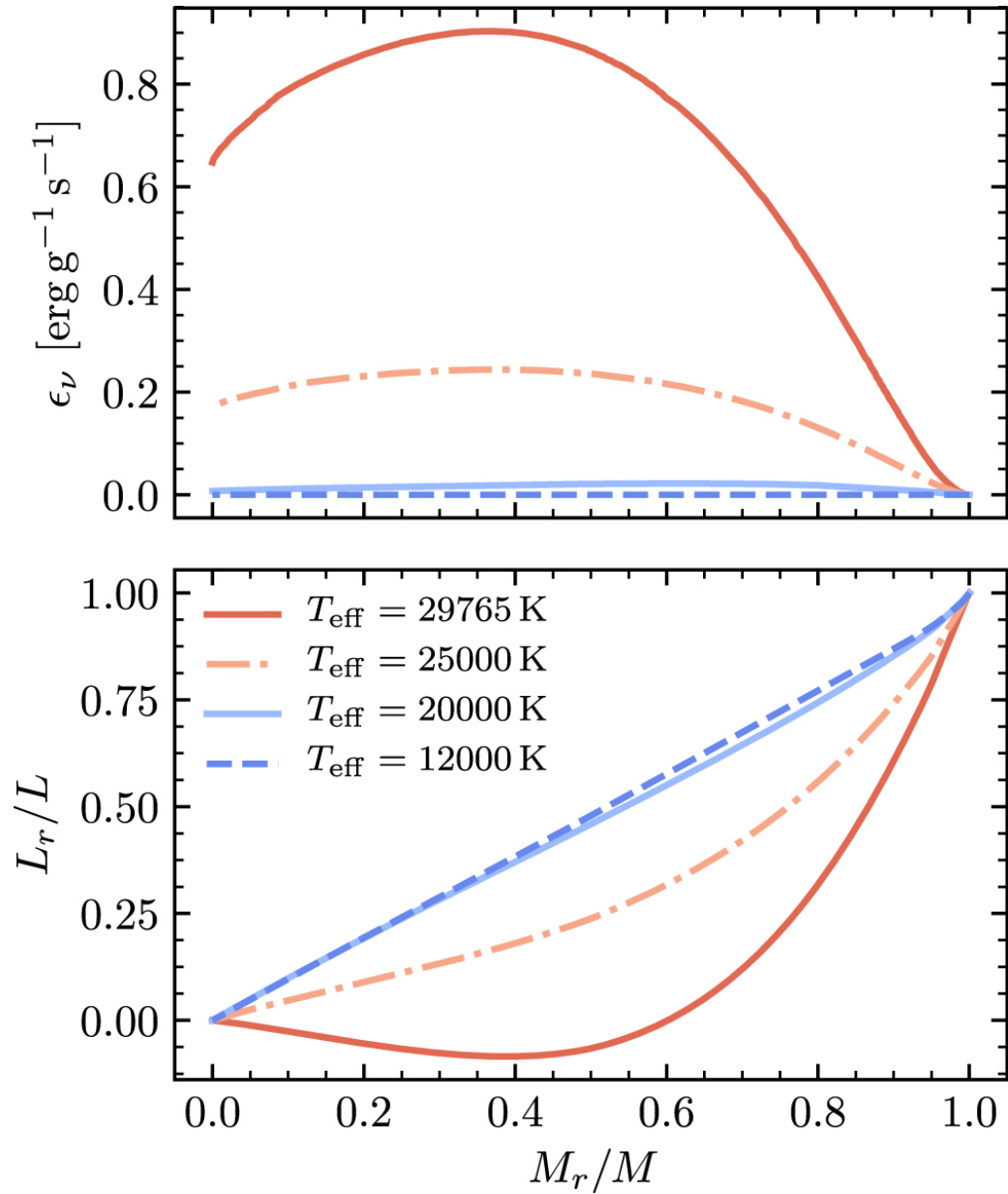
Figure 5. from The Impact of White Dwarf Luminosity Profiles on Oscillation Frequencies null 2018 APJL 867 L30 doi:10.3847/2041-8213/aae70f https://dx.doi.org/10.3847/2041-8213/aae70f © 2018. The American Astronomical Society.
