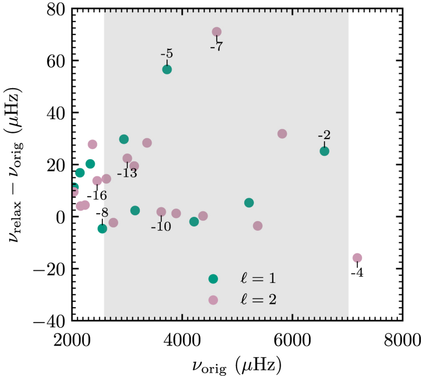
Figure 3. from The Impact of White Dwarf Luminosity Profiles on Oscillation Frequencies null 2018 APJL 867 L30 doi:10.3847/2041-8213/aae70f https://dx.doi.org/10.3847/2041-8213/aae70f © 2018. The American Astronomical Society.
