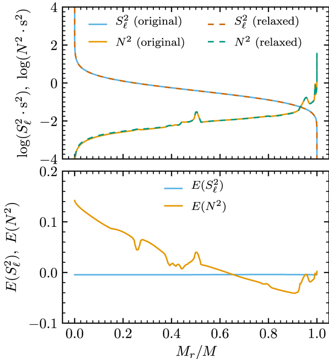
Figure 2. from The Impact of White Dwarf Luminosity Profiles on Oscillation Frequencies null 2018 APJL 867 L30 doi:10.3847/2041-8213/aae70f https://dx.doi.org/10.3847/2041-8213/aae70f © 2018. The American Astronomical Society.
