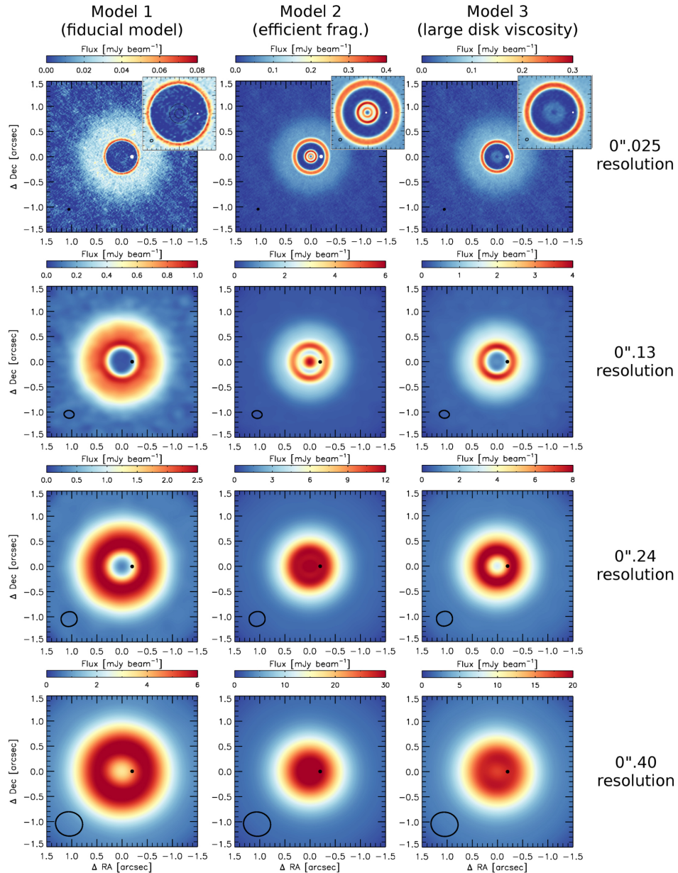
Figure 8. from Diverse Protoplanetary Disk Morphology Produced by a Jupiter-mass Planet null 2018 APJL 864 L26 doi:10.3847/2041-8213/aadd51 https://dx.doi.org/10.3847/2041-8213/aadd51
