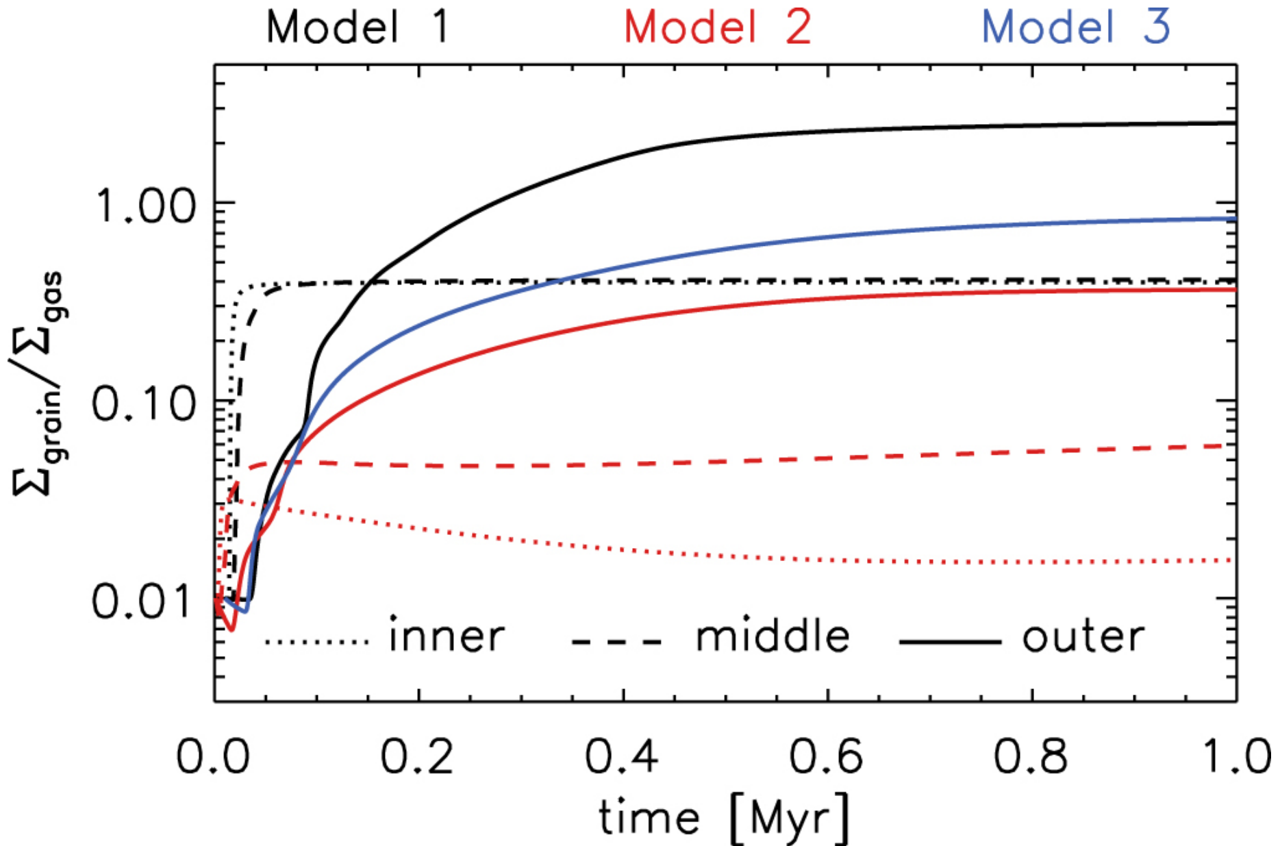
Figure 7. from Diverse Protoplanetary Disk Morphology Produced by a Jupiter-mass Planet null 2018 APJL 864 L26 doi:10.3847/2041-8213/aadd51 https://dx.doi.org/10.3847/2041-8213/aadd51 © 2018. The American Astronomical Society. All rights reserved.
