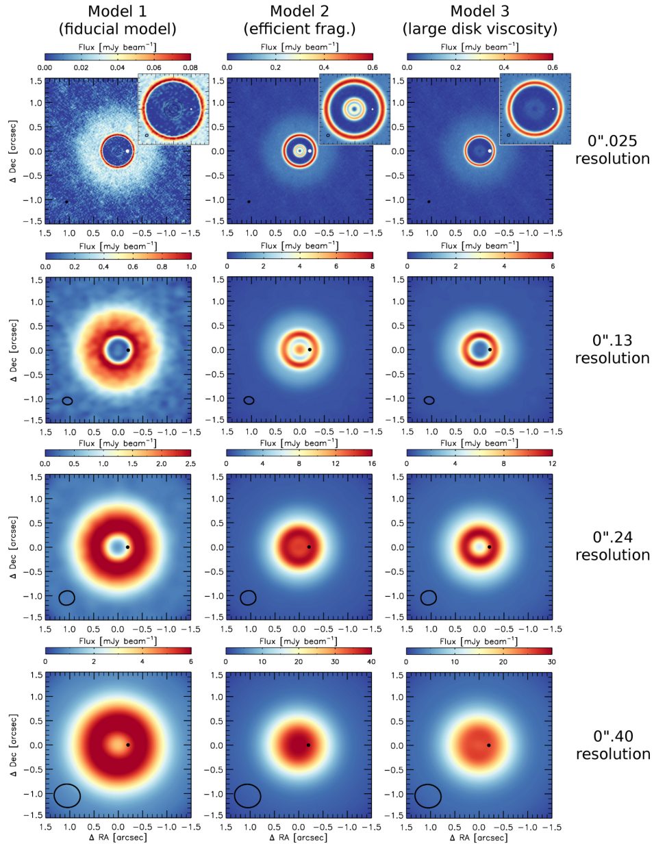
Figure 6. from Diverse Protoplanetary Disk Morphology Produced by a Jupiter-mass Planet null 2018 APJL 864 L26 doi:10.3847/2041-8213/aadd51 https://dx.doi.org/10.3847/2041-8213/aadd51
